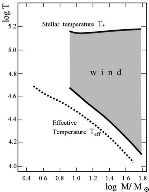
Fig. 27.16 Relations between the temperatures T_* , T_{\text{eff}} and the actual masses of WC/WO stars for the \dot{M} rates by de Jager et al. [271]. The dotted lines are for rates twice larger. Adapted from D. Schaerer and the author [511]
