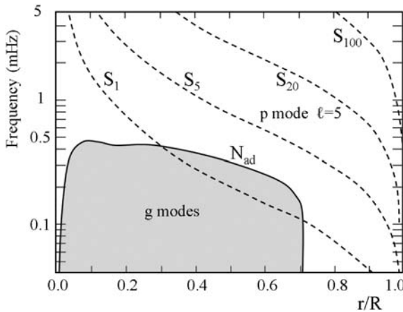
Fig. 16.1 Variations of the Brunt–Väisälä N_{\text{ad}} and of the Lamb S_{\ell}(r) frequencies for various values of \ell as a function of the radius in the solar model. The g-mode trapping region is indicated by a gray area. The outer convection extends from this zone to the surface. The trapping regions are also limited by the acoustic cutoff frequency (cf. Fig. 16.8). Adapted from J. Christensen-Dalsgaard [131]
