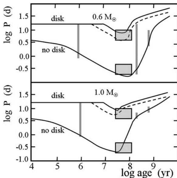
Fig. 21.6 Evolution of the rotation periods as a function of time for 0.6 M_{\odot} and 1.0 M_{\odot} models. In each diagram, the upper continuous line applies to a starting period of 16 days, a disk is present with a lifetime of 10^7 yr ( continuous line ) and with 3 \times 10^6 yr ( broken line ); the lower curve applies to a starting period of 4 days, no disk is present. The lower and upper boxes represent the observed period for the fast and slow rotators in \alpha Per and the Pleiades. The gray bar at 10^6 yr represents the observed range of periods in T Tauri stars. The gray bars at 2.5 \times 10^8 and 6 \times 10^8 yr represent data in NGC 3532 and the Hyades for the corresponding masses. Adapted from S. Barnes, S. Sofia & M. Pinsonneault [36]
