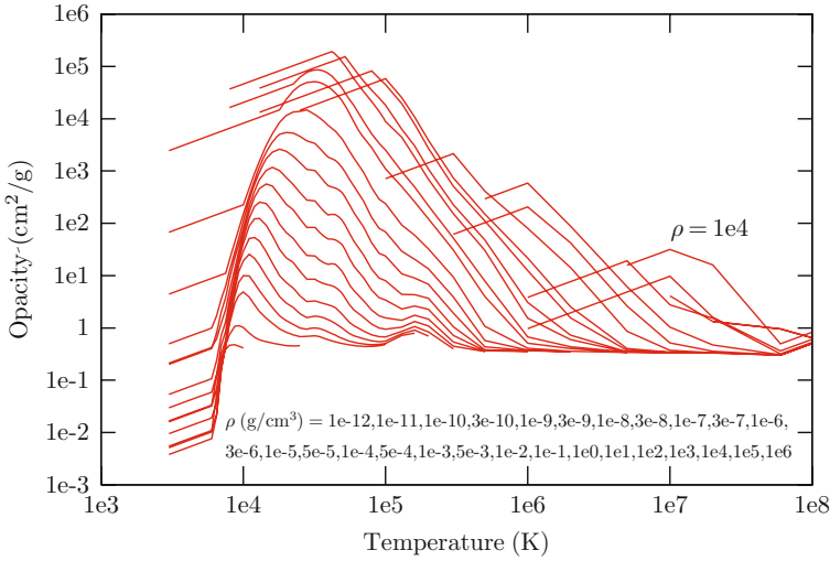
Fig. 8.2 Opacities with a difference of 25 years. Top: opacities from A.N. Cox in 1983 [144] as a function of T and \rho for X = 0.70 and Z = 0.02 . Curves nb. 3, 1, 9, 6 on the right of the peak correspond to \rho = 10^4, 10^2, 1.0, 10^{-2} \text{ g cm}^{-3} . Curve 3 at the max. is for 10^{-3} \text{ g cm}^{-3} . Curves 1, 7, 3 and 1 on the left of the peak correspond to \rho = 10^{-4}, 10^{-6}, 10^{-8}, 10^{-10} \text{ g cm}^{-3} . Bottom: opacities in 2008 provided by A.N. Cox and A.T. Boothroyd from OPAL [493] for the new solar abundances [20], Appendix A.3. The straight lines on the left of each curve indicate where usual stellar conditions end. Courtesy by A.N. Cox
