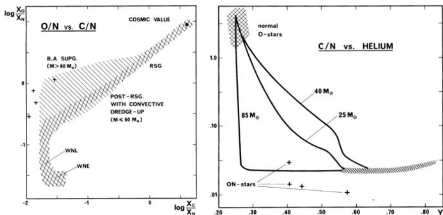
Fig. 27.12 Left : relation between the surface O/N and the C/N ratios for massive stars. Right : relation between the surface C/N and the He contents. Values are in mass fractions. Crosses represent ON stars. From the author [343]
