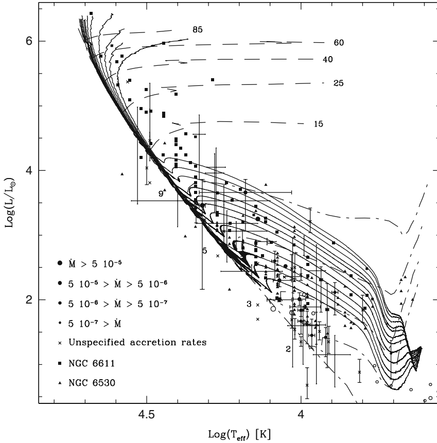
Fig. 20.6 Comparison of various birthlines with accretion rates equal from bottom to top to 0.1, 0.15, 0.2, 0.3, 0.5, 0.75, 1.0, 1.25, 1.75, 2.5, 3.5 and 5.0, the case illustrated by the data of Table 20.2. Pre-MS tracks at constant mass are indicated by dot-dashed lines and post-MS tracks of high masses by dashed lines. Numbers indicate the stellar masses. The observations are Ae/Be Herbig and T Tauri stars with different values of \dot{M}_{\text{accr}} and sources. From P. Norberg and the author [443]
