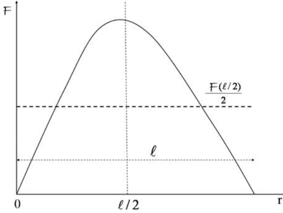
Fig. 5.2 Schematic representation of the force on a moving element
