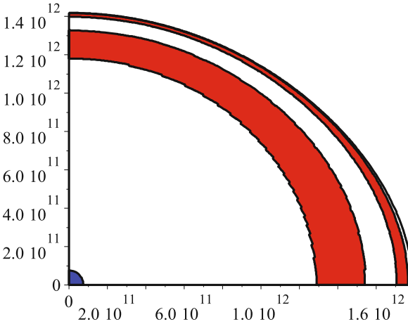
Fig. 6.7 Two-dimensional representation of the convective zones ( dark areas ) in a model of 20 M_{\odot} with X = 0.70 and Z = 0.020 at the end of MS evolution with (\Omega/\Omega_{\text{crit}} = 0.94) , with an account of only \nabla_{\text{rad}} and \nabla_{\text{ad}} . The axis units are cm. From the author, C. Georgy and G. Meynet [357]
