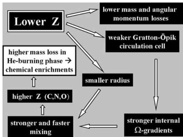
Fig. 29.7 Main effects of rotation and mass loss at very low Z
