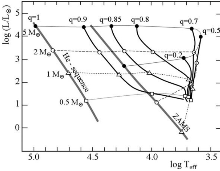
Fig. 24.3 Generalized MS in the HR diagram. Models of various total mass with He cores representing different mass fraction q are shown. Thick lines connect models with the same fraction q , thin lines connect models of the same total mass. The usual MS and He sequence are shown by thick gray lines . The envelope composition is X = 0.68, Z = 0.02 . Adapted from P. Giannone et al. [205, 285]
