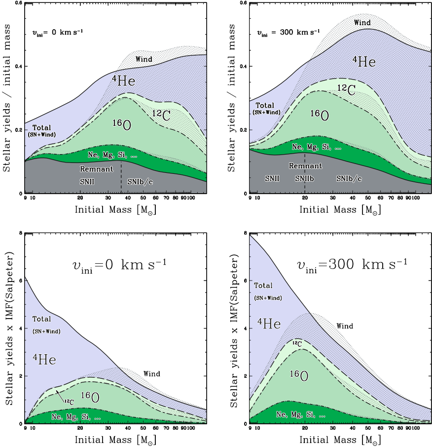
Fig. 28.8 Mass fractions ejected as a function of the initial masses for models with X = 0.705 , Z = 0.020 . The mass loss rates of all models are from Vink et al. [604, 605], de Jager et al. [271] and Nugis and Lamers [445] for WR stars. Anisotropic winds are accounted for M > 40 M_{\odot} . The wind contributions are shown with dotted areas. For ^4\text{He} , the wind contribution may be larger than the total yield, because some ^4\text{He} is destroyed in the supernova. Upper left: without rotation. Upper right: with rotation. Lower left and right: the same with convolution by a Salpeter's initial mass function dN/dM \sim M^{-2.35} . From R. Hirschi et al. [252]
