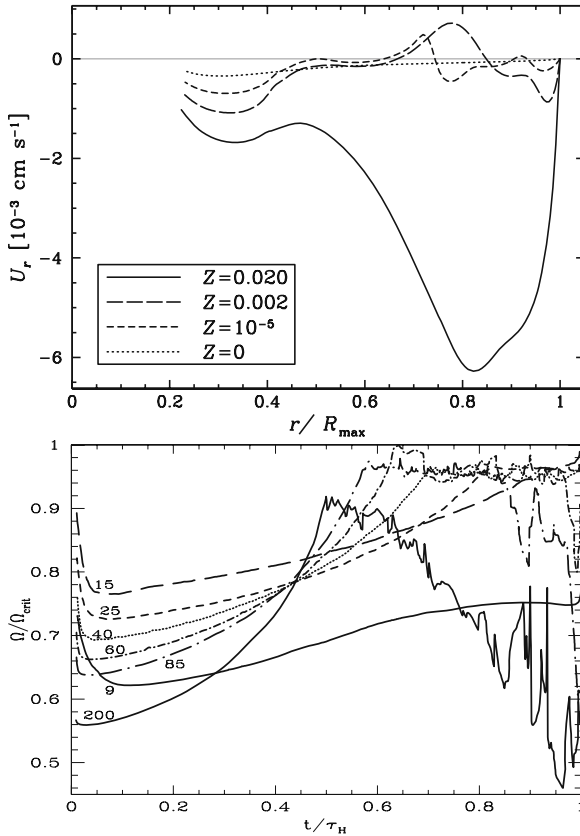
Fig. 29.6 Top : values of the velocity of meridional circulation U_2(r) in 20 M_\odot models of different Z . Bottom : evolution of the \Omega/\Omega_{\text{crit}} ratio during the MS phase of various masses at Z = 0 . All the models start with v_{\text{eq}} = 800 \text{ km s}^{-1} , except the 9 M_\odot which starts with 500 \text{ km s}^{-1} . From G. Meynet, S. Ekström and A. Maeder [175]
