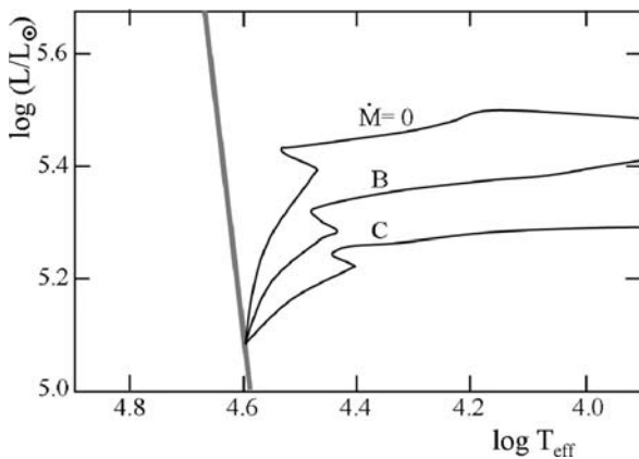
Fig. 27.4 MS tracks of a 30 M_{\odot} star with X = 0.70 and Z = 0.03 without mass loss and with \dot{M} = NL/c^2 (14.1) in CGS units for N = 70 (B) and N = 140 (C)
