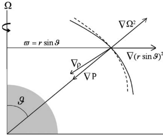
Fig. 11.1 In a star with shellular rotation, the surfaces of equal density ( dashed line ) and pressure (isobar, continuous line ) do not coincide. The star is baroclinic. The gradient of density has a horizontal component (i.e. on the isobar) and the same for the T gradient. Adapted from Zahn [632]
