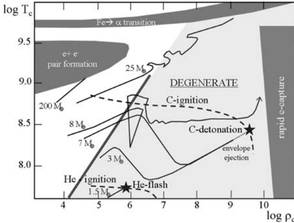
Fig. 26.10 Evolution of central conditions for different masses with indications of instability domains (Sect. 7.8), the Fe- \alpha transition indicates the photodisintegration of Fe nuclei into \alpha particles. The degenerate region is light gray. Dashed lines show the place where nuclear energy generation rates balance neutrino losses. Adapted from T.J. Mazurek and J.C. Wheeler [393]
