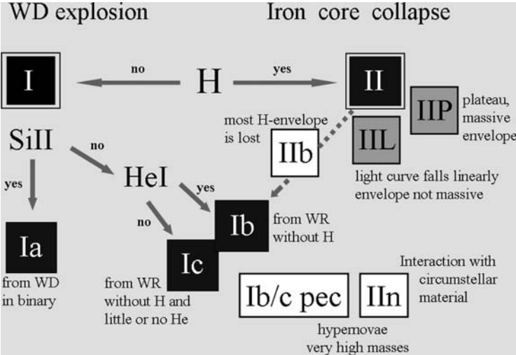
Fig. 28.9 Classification and main characteristics of supernovae. The main groups are in black squares. Adapted from M. Turatto [581]
