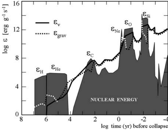
Fig. 28.6 Evolution of the rates of nuclear energy (gray), of neutrino emission (continuous line) and of gravitational energy (dotted line) for a 20 M_{\odot} star with Z = 0.02 . Same remark as for Fig. 28.5. Adapted from Hirschi et al. [251]
