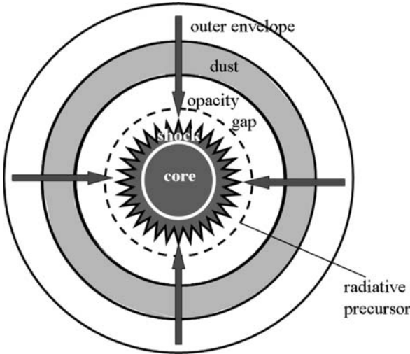
Fig. 19.3 Schematic structure of a protostar in the strong spherical accretion phase. The radii of the various shells are 10^{17} cm for the cloud boundary, 10^{14} cm for the outer edge of the dust layer, 10^{13} cm for the dust destruction front and 10^{11} cm for the accretion shock. Adapted from S.W. Stahler, F.H. Shu and R.E. Taam [549]
