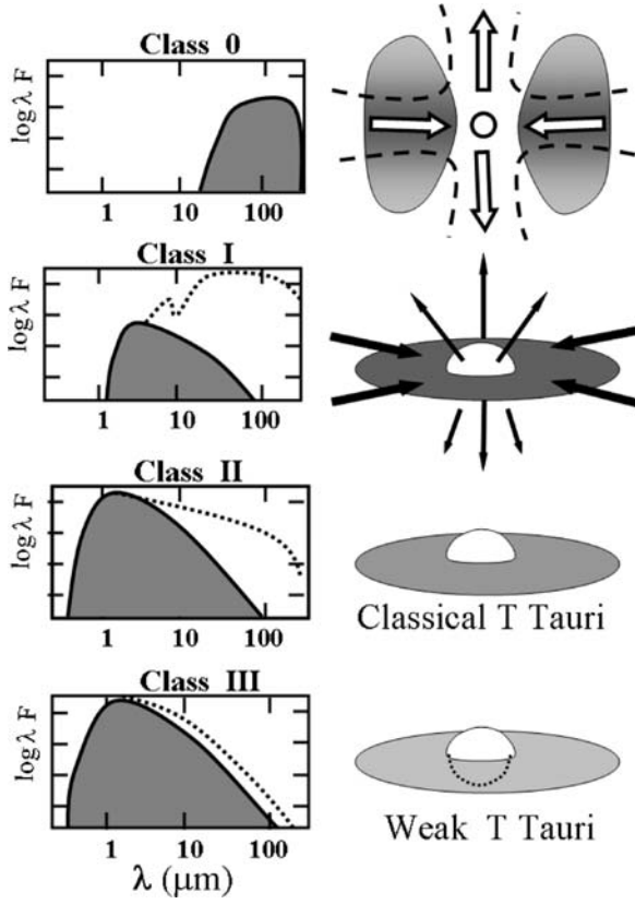
Fig. 19.1 The sequence of the various classes of accretion disks. On the left, a simplified representation of the stellar flux F is given (shaded area), the contribution of the disk is indicated by a dotted line. On the right a schematic representation of the object is given. Adapted from André [11]
