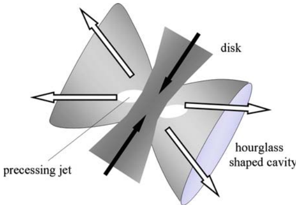
Fig. 22.2 Schematic picture of a protostellar disk with massive bipolar outflows. The central protostar is obscured by a large slowly rotating disk with a diameter of 20\,000\,\text{AU} and a mass of 100\,M_{\odot} . A fraction of the infalling material is accelerated into bipolar precessing jets. The high-velocity wind forms an hourglass cavity in the ambient medium. Adapted from Chini [126]
