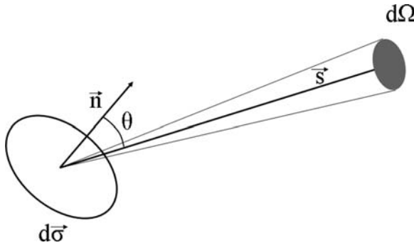
Fig. C.1 The geometrical parameters associated to a radiation beam
