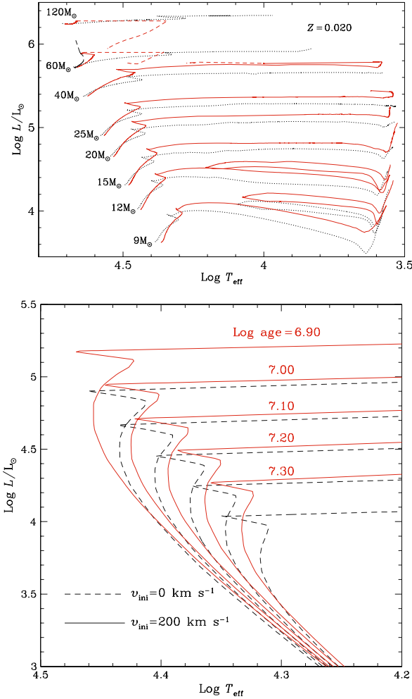
Fig. 27.8 Top: tracks at Z = 0.02 for non-rotating stars ( dotted lines ) and for stars with initial velocities of 300 \text{ km s}^{-1} ( continuous lines ), corresponding to a MS average \bar{v} = 160\text{--}235 \text{ km s}^{-1} . Bottom: isochrones of \log(\text{age}) = 6.9 to 7.3 for zero rotation ( dashed lines ) and for initial v = 200 \text{ km s}^{-1} ( continuous lines ). The dashed line of \log(\text{age}) = 6.9 is close to the continuous line with \log(\text{age}) = 7.0 . From G. Meynet and the author [409]
