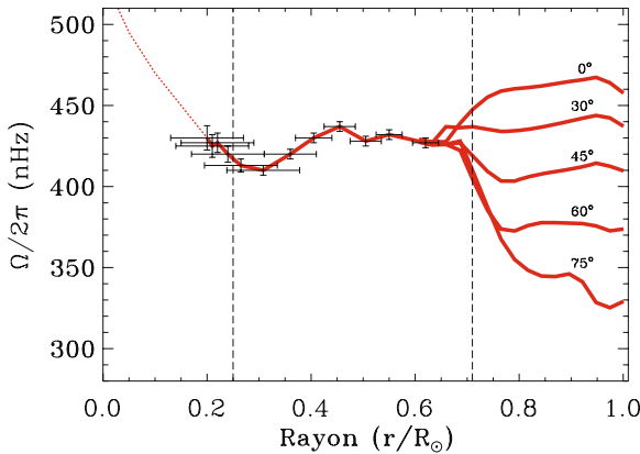
Fig. 16.20 The internal value of the angular velocity \Omega as a function of solar radius in the Sun from the acoustic modes in helioseismic observations. In the outer layers, the curves are different according to the latitude (zero degree corresponds to the equator). The data are obtained from the inversion technique on modes \ell \leq 25 using a series of 2088 days. Below 0.2 R_{\odot} the dotted curve indicates the result suggested by gravity modes using the GOLF experiment on SOHO (ESA and NASA); this part is however still uncertain. Data from [200, 583]. Courtesy of S. Turck-Chièze
