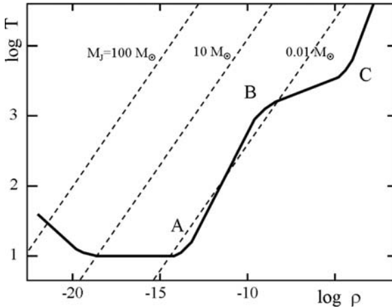
Fig. 19.4 Evolution of temperature and density at the center of a forming star evolving at a constant mass of 1 M_{\odot} [576]. Point A marks the end of the isothermal phase. A–B is the adiabatic phase of molecular gas. B–C is the transition from molecular to neutral gas and from neutral to ionized gas. C marks the beginning of the adiabatic phase of ionized gas. Adapted from P. Bodenheimer [51]
