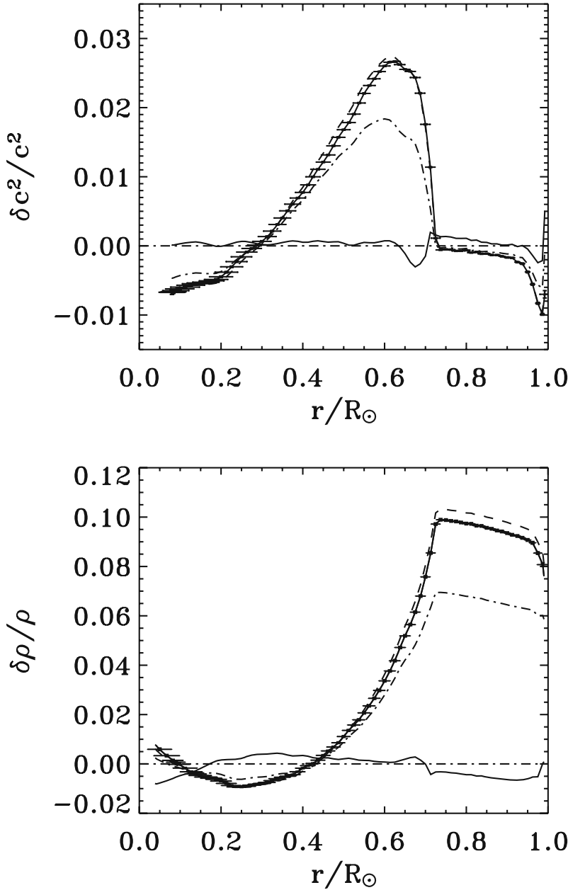
Fig. 16.12 Upper: the relative differences (squared) of the sound speed between the helioseismic observations with GOLF and MDI aboard SOHO (ESA and NASA) for three solar models with slightly different Z/X ratios. The full line with error bars is that based on new CN ( lower ); CNO abundances from Asplund [19]. The continuous line close to horizontal is not a physical model, but a so-called seismic model adjusted on observational constraints. The other curves correspond to different equations of state [152, 494, 495]. Lower: the equivalent in terms of density differences [582, 583]. Courtesy of S. Turck-Chièze
