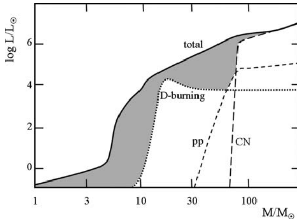
Fig. 23.3 Evolution as a function of the growing mass on the birthline at Z = 0 of the maximum of the interior luminosity ( continuous line ), of the contribution of D burning ( dotted line ), of the pp chain ( short-dashed line ) and of the CN cycle ( long-dashed line ). This refers to the reference accretion rate of 4.4 \times 10^{-3} \text{ M}_{\odot} \text{ yr}^{-1} . The difference between the total and nuclear luminosities is due to gravitational contraction ( gray area ). Adapted from K. Omukai and F. Palla [448]
