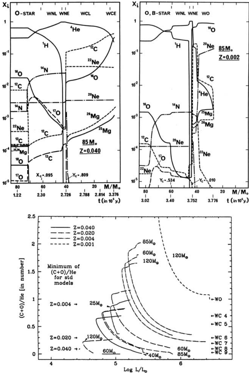
Fig. 27.17 Top : comparisons of extreme cases of evolution of surface abundances for very massive stars at Z = 0.04 and Z = 0.002 as a function of age and remaining mass. From the author [346]. Bottom : the (C+O)/He ratios in WC stars as a function of L for different Z and initial masses. The scale of WC subtypes by Smith and Hummer [538] is given. From the author and G. Meynet [365]
