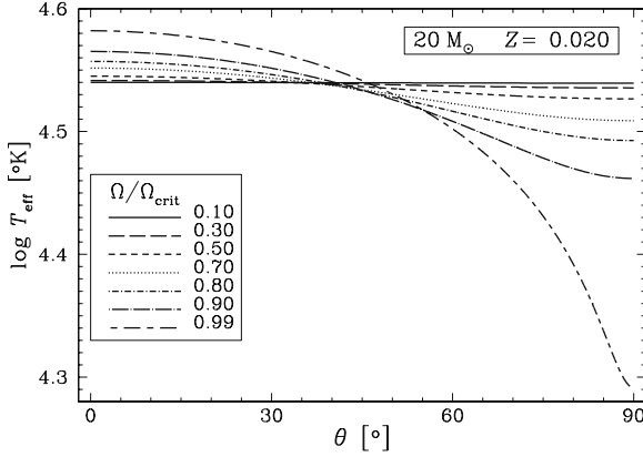
Fig. 4.1 Illustration of the von Zeipel theorem. The local T_{\text{eff}} as a function of the colatitude \vartheta for models of 20 M_{\odot} on the ZAMS with various ratios \Omega/\Omega_{\text{crit}} of the angular velocity to the critical value. The stellar shape is shown in Fig. 2.2. Courtesy G. Meynet
