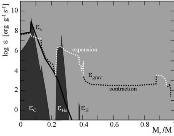
Fig. 28.5 Distribution of the energy production rates \epsilon per unit of mass inside a 20 M_{\odot} star ( Z = 0.02 ) at the end of the central C burning. The darker areas show the nuclear energy production, the thick continuous line gives the \nu emission (counted positive) and the dotted line the gravitational energy, positive (contraction) in black, negative (expansion) in white. Adapted from Hirschi et al. [251]
