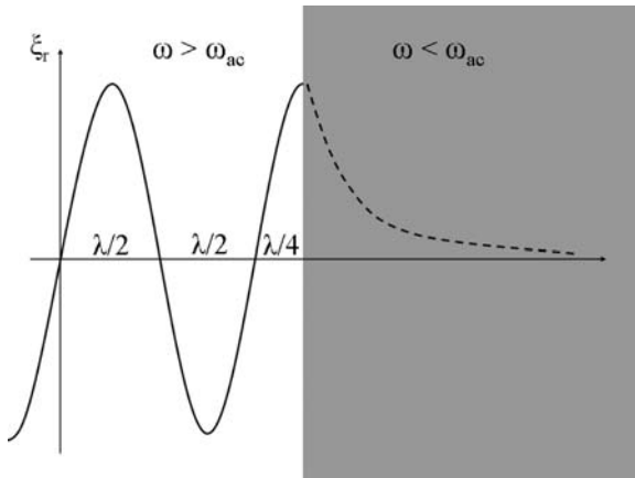
Fig. 16.3 Schematic representation of the boundary of a propagation zone of p modes. There is an integer number of \lambda/2 , plus a fraction of \sim (1/4)\lambda in the cavity. At the boundary, the stationary waves match an exponential decrease
