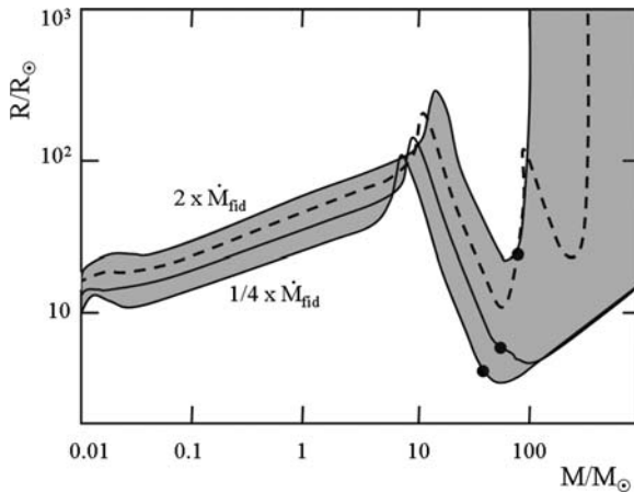
Fig. 23.2 Mass–radius relations for Z=0 stars on the birthline for different accretion rates 2, 1, (1/2) and (1/4) \dot{M}_{\text{ref}} (gray zone), where the reference value \dot{M}_{\text{ref}} = 4.4 \times 10^{-3} M_{\odot} \text{ yr}^{-1} (dashed line). The beginning of the H burning through the CN cycle is indicated by black dots. Adapted from K. Omukai and F. Palla [448]
