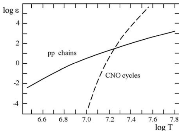
Fig. 25.2 Energy generation rates ( \text{erg g}^{-1} \text{s}^{-1} ) by the pp chains and by the CNO cycles as a function of T for \rho = 100 \text{ g cm}^{-3} , X = 0.70 and X_{\text{CNO}} = 10^{-2}
