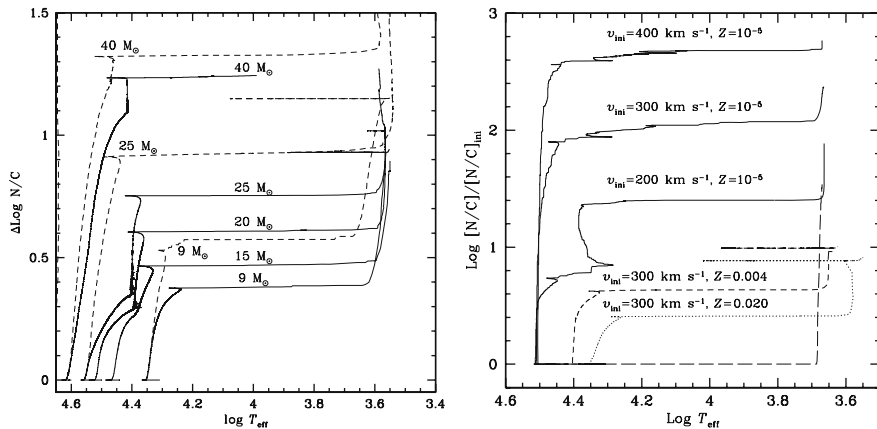
Fig. 27.13 Left : evolutionary tracks in the plot \Delta \log(N/C) (change with respect to the initial N/C ratio) vs. \log T_{\text{eff}} for various initial masses with Z = 0.02 with initial velocities 300 \text{ km s}^{-1} (continuous lines). The dashed lines show the tracks with different model assumptions [409]. Right : excesses N/C in log scale for a 9 M_{\odot} star at different metallicities and rotation velocities. The long-dashed line, at the bottom, corresponds to a non-rotating 9 M_{\odot} stellar model at Z = 10^{-5} . From G. Meynet and the author [410, 411]
