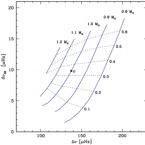
Fig. 16.17 Asteroseismic diagram for solar-type stars with solar composition X = 0.718 , Z = 0.014 during their MS evolution. The evolution of different masses are indicated by continuous lines. The dotted lines show the loci with the same central H content X_c . The model with 1.2 M_{\odot} is followed up to the appearance of a convective core. The solar observations are indicated. From P. Eggenberger [169]
