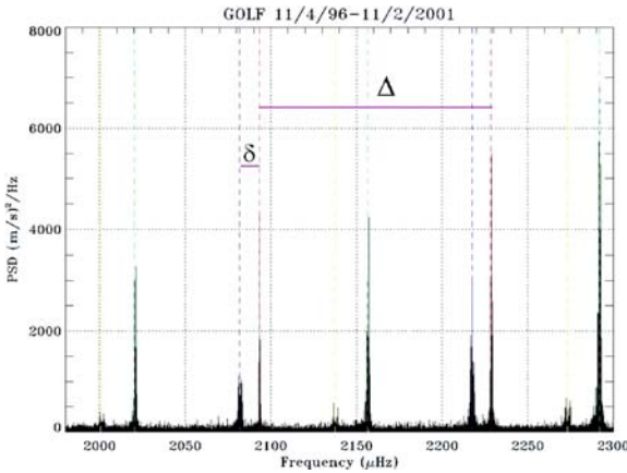
Fig. 16.10 Details from the solar power spectrum from GOLF illustrating the definitions of the large separation \Delta \nu (noted \Delta ) and of the small separation \delta \nu_{02} (noted \delta ). Figure from the GOLF experiment on the SOHO satellite of ESA and NASA; see [195]. Courtesy of S. Turck-Chièze
