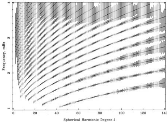
Fig. 16.7 The solar p modes observed at Big Bear Solar Observatory from K.G. Libbrecht and M.F. Woodard [325, 327]. Each parabolic line corresponds to a fix number n ; the lowest line is for n = 1 . The small vertical line show the 1\sigma error bar enlarged by a factor 10^3 . With permission
