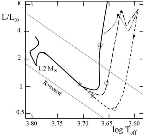
Fig. 20.12 The continuous thick line shows a pre-MS evolution for a constant 1.2 M_{\odot} star. The three other tracks start at the top of the Hayashi line with M = 0.5 M_{\odot} . The dotted line shows a fast initial accretion; the star reaching its final mass in 10^6 yr. The long-broken track is for a decreasing accretion rate. The short-broken line shows the track for a negligible accretion until 10^6 yr and a large after that. The black squares indicate the return to radius contraction as the main energy source, after some expansion due to D burning. The ellipses mark the beginning of a radiative core; this is about the point where Li is burning. The stars indicate the end of accretion. At point marked 1.2 M_{\odot} , the star reaches the ZAMS. Loci of constant radius are indicated. Adapted from Siess [529]
