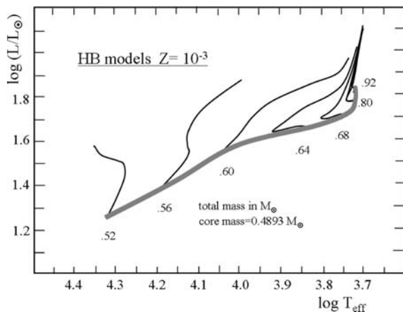
Fig. 26.12 Evolutionary tracks for horizontal branch stars with initial helium content Y = 0.23 , Z = 0.001 , core mass 0.4893 M_{\odot} and indicated total masses. Adapted from S. Yi, Y.-W. Lee and P. Demarque [625]
