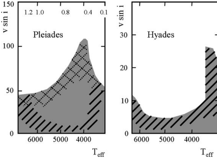
Fig. 21.5 Distributions of the rotational velocities in the Pleiades and Hyades as a function of T_{\text{eff}} . The heavy shaded areas indicate where most stars are lying; the lighter shaded area shows the location of a significant fraction of Pleiades stars. The gray areas indicate regions where stars may be present. The scale at the top of the left diagram is an indicative mass scale. Adapted from J. R. Stauffer [550]
