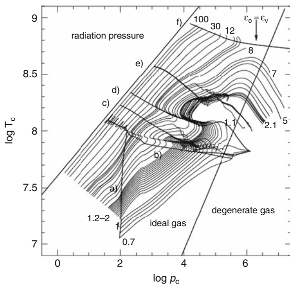
Fig. 29.2 Evolution of central conditions at Z = 0 (models of Fig. 29.1). The domains of different equations of state are indicated. Line (a) shows the onset of the pp reactions, (b) the onset of the 3\alpha reaction which permits the CNO cycles to start, (c) the end of core H burning, (d) the central He ignition, (e) the end of the core He-burning phase and (f) the place where the neutrinos losses compensate for C burning. From P. Marigo, L. Girardi, C. Chiosi and P.R. Wood [377]
