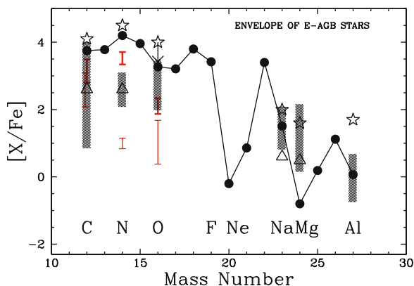
Fig. 26.25 Average chemical composition of the envelopes of E-AGB stars. The continuous line with black circles applies to a 7 M ⊙ model at Z = 10^{-5} ( [\text{Fe}/\text{H}] = -3.6 ) with an initial velocity v_{\text{ini}} = 800 \text{ km s}^{-1} . The vertical error bars indicate the ranges of values for CNO elements in the models [410] with initial masses between 2 and 7 M ⊙ at Z = 10^{-5} ; the thick and thin bars correspond to rotating ( v_{\text{ini}} = 300 \text{ km s}^{-1} ) and non-rotating models. The observed abundances of extremely metal-poor stars are shown by hatched areas (observations by Plez and Cohen [473] with triangles, by Frebel et al. [186]) with stars). From G. Meynet et al. [407]
