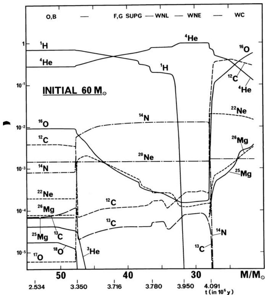
Fig. 27.11 Evolution of the surface abundances in mass fractions X_i for a 60 M_{\odot} star ( X=0.70 , Z=0.02 ) as a function of the remaining mass and age. The age zero is on the ZAMS. Indications of the corresponding stages. From the author [345]
