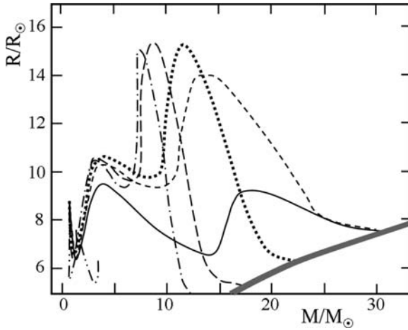
Fig. 22.11 Relation between radius and masses for stars on the various birthlines calculated with (19.26). The notation of the lines is the same as in Fig. 22.8. The thick continuous line shows the relation for the ZAMS [464]
