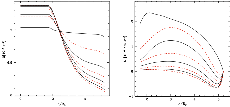
Fig. 11.6 Left : initial evolution of the angular velocity \Omega(r) in a 20 M_{\odot} star with v_{\text{ini}} = 300 \text{ km s}^{-1} (standard abundance). Starting from a nearly flat profile, the solutions rapidly converge toward an equilibrium profile of differential rotation. The time interval between two consecutive curves is 19200 years. Right : U_2(r) the vertical component of the meridional circulation velocity. Time proceeds from top to bottom. From Meynet and the author [409]
