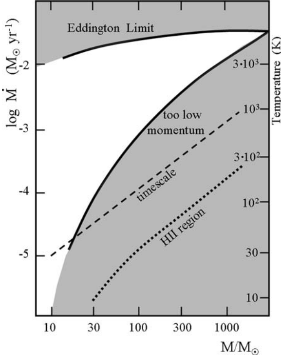
Fig. 22.4 Various limits on the accretion rates as a function of the protostellar mass. The white area is the region where accretion is permitted. The upper limit indicates where the inflow rate becomes supra-Eddington for electron scattering opacity. The limit below which the momentum in the inflow is smaller than the momentum of the radiation field is indicated (Sect. 22.3.3). Below the limit labeled “timescale” the formation timescale would be longer than 10^6 yr. Below the limit noted “HII region” an HII region expands beyond the dust destruction radius and prevents accretion. Adapted from M.G. Wolfire and J.P. Cassinelli [616]
