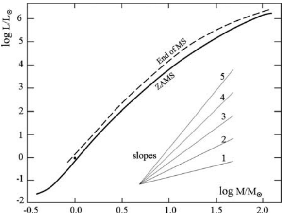
Fig. 25.6 The mass-luminosity relation for stars from 0.4 to 120 M_{\odot} on the ZAMS and at the end of the MS phase for models with X = 0.68 and Z = 0.02 . The dot shows the solar values. Some slopes are shown [513]
