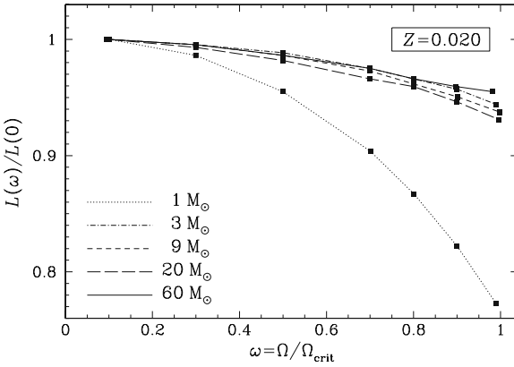
Fig. 4.2 Relative variations of the total stellar luminosity for models of various masses on the ZAMS at Z = 0.02 as a function of the rotation parameter \omega = \Omega/\Omega_{\text{crit}} . From S. Ekström et al. [176]
