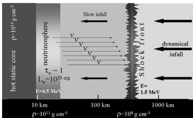
Fig. 28.11 Schematic illustration of the shock front, neutrinosphere and neutron core during core collapse
