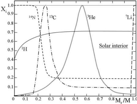
Fig. 25.9 Internal distribution of the abundance in mass fractions for some elements in the Sun. Except for H, the abundances are normalized to the maximum values reached in the Sun: X(^{14}\text{N}) = 3.34 \times 10^{-3} at the center, X(^{13}\text{C}) = 3.82 \times 10^{-4} at M_r/M = 0.249 , X(^3\text{He}) = 3.448 \times 10^{-3} at M_r/M = 0.550 , X(^7\text{Li}) = 7.37 \times 10^{-9} at the surface. ^7\text{Li} is destroyed for T > 2.5 \times 10^6 K, which corresponds to M_r/M = 0.968 and r/R = 0.663 . From data by C. Charbonnel [119]
