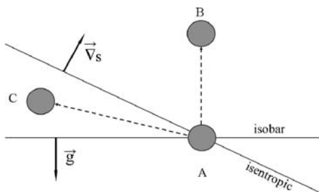
Fig. 12.7 Illustration of the baroclinic instability. The gravity is perpendicular to the isobar, the line of constant entropy is also shown. A displacement from A to B is stable, while from A to C it is unstable, i.e., the fluid element is not brought back
