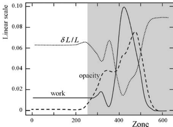
Fig. 15.1 The relative excess of luminosity \delta L/L , the cumulative work and the opacity in a Cepheid model of 7 M_{\odot} as a function of the zoning of the outer layers. The stellar surface is on the left, the white area is the atmosphere with optical depth < 2/3 , the gray area is the optically thick envelope. The cumulative work is the sum of the work, positive or negative, from the inner zone (600) up to the surface. As the integrated work up to the surface is positive, the star is unstable. Adapted from Schaller [512]
