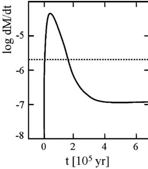
Fig. 19.2 Accretion rate as a function of time for a gravo-turbulent fragmentation from Schmeja and Klessen [518] predicting an initial peak in the accretion rate. The horizontal dotted line corresponds to (19.24) with a numerical coefficient 0.975
