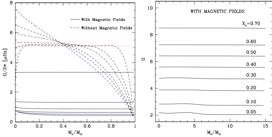
Fig. 13.5 Left: rotation profiles as a function of the Lagrangian mass in evolving solar models with and without magnetic field [172] (magnetic braking at the surface is accounted for). The dotted line indicates the initial profile. As evolution proceeds, the global profile for the case without magnetic field becomes steeper, while with magnetic field \Omega is almost constant, its value goes down strongly in time due to braking at the stellar surface. Right: rotation profiles at various stages of evolution (labeled by the central H content X_c ) of a 15 M_\odot model with X = 0.705 , Z = 0.02 , an initial velocity of 300 \text{ km s}^{-1} and magnetic field. The evolution of velocity in a model without field is shown in Fig. 11.8. From the author and G. Meynet [369]
