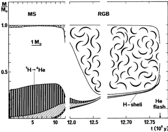
Fig. 25.10 Evolution of the internal structure of a 1 M_{\odot} star with X = 0.70 and Z = 0.02 from the ZAMS to the He flash. The properties are represented according to the mass fraction as a function of time. Cloudy regions represent convective zones. Vertically hatched regions show the region where the nuclear energy generation rate \epsilon is between 1 and 10 \text{ erg g}^{-1} \text{ s}^{-1} and diagonally hatched regions above 10 \text{ erg g}^{-1} \text{ s}^{-1} . From Maeder and Meynet [363]
