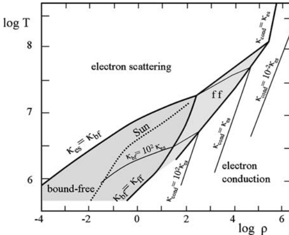
Fig. 8.3 Indications of the dominant opacity sources in the \log T vs. \log \rho diagram. The location of the solar internal structure is indicated by a thick dotted line . The electron conduction is expressed in terms of the electron scattering opacity \kappa_{es}
