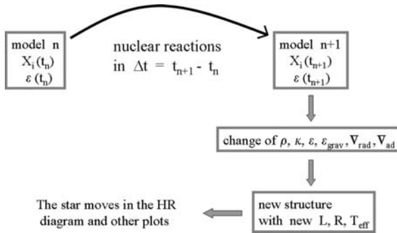
Fig. 24.1 Steps in stellar evolution
