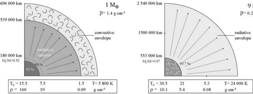
Fig. 25.5 Schematic structure of the Sun and a star of 9 M_{\odot} on the main sequence with indications of T and \rho . Cloudy regions indicate convection. The percentages indicate the fraction of the total energy produced
