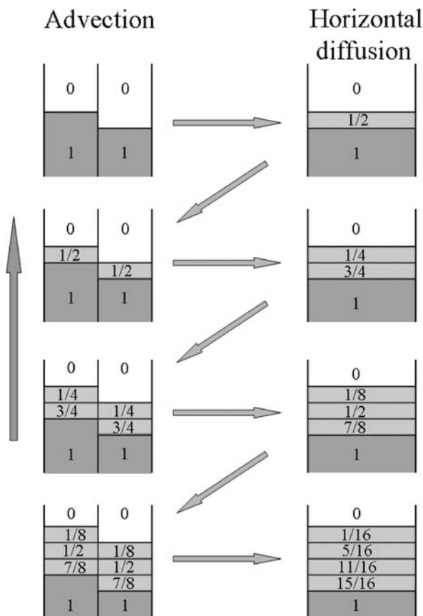
Fig. 11.10 Schematic illustration of the combination of the effects of circulation and horizontal turbulence. The very left column is moving up, at each time step the horizontal turbulence mixes the layers. This makes a distribution like the error function, showing that the combination of both motions acts as a diffusion as far as the mixing of elements is concerned. Adapted from slides by J.-P. Zahn
