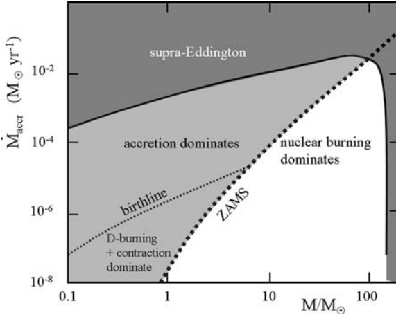
Fig. 22.3 Domains of accretion rates vs. masses. The heavy dotted line shows for stars on the ZAMS the place where the accretion luminosity is equal to the stellar luminosity. The thin dotted line shows the place where the accretion luminosity is equal to the contraction+D burning luminosity on the birthline. The darker domain shows the region where the accretion rate is such that the sum of the stellar and accretion luminosity is larger than the Eddington luminosity, assuming electron scattering opacity. Adapted from H.W. Yorke [627]
