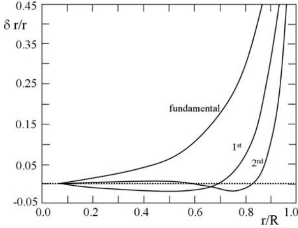
Fig. 15.2 The perturbations of radius for the fundamental mode, the first and second overtones as functions of radius in \alpha Vir, a 11 M_{\odot} Main Sequence star. Each mode is normalized to 1.0 at the surface. Adapted from A.N.Cox [144]
