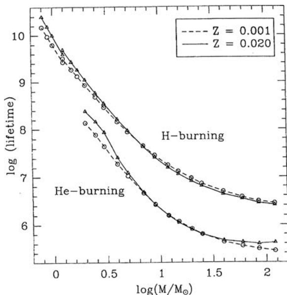
Fig. 26.4 The lifetimes (yr) for the H- and He-burning phases as a function of the mass on the ZAMS for Z = 0.02 , Y = 0.30 and for Z = 0.001 and Y = 0.243 , with an overshooting of 0.20 H_p from the core. From G. Schaller et al. [513]
