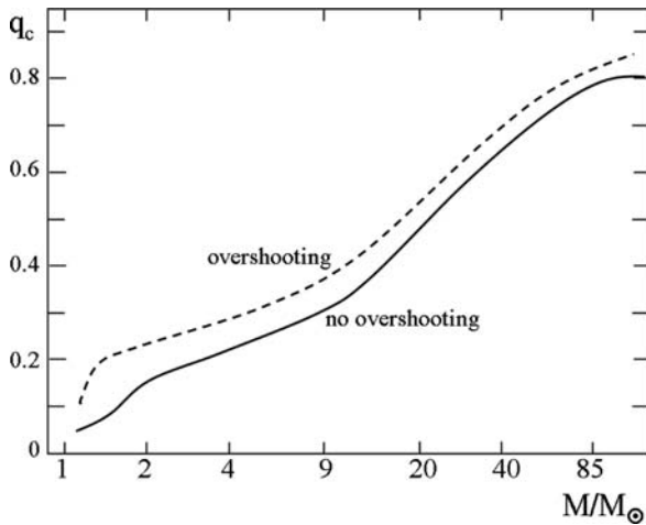
Fig. 6.4 The mass fraction of the convective cores without and with an overshooting d_{\text{over}}/H_P = 0.25 . If the size r_c of the core is smaller than H_P , d_{\text{over}} = 0.25 r_c . At 1.15 M_\odot , d_{\text{over}}/H_P = 0.125 . From the author [363]
