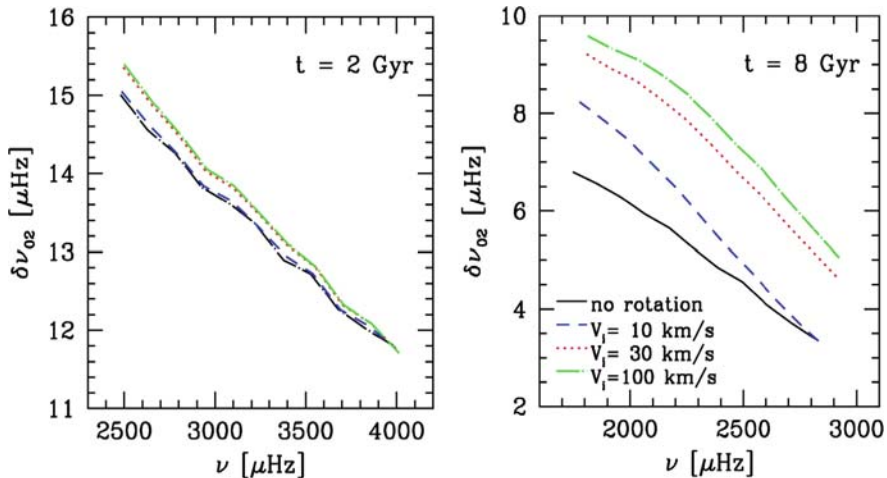
Fig. 16.21 The small separation \delta\nu_{02} vs. frequency at two different stages with an age of 2 Gyr and 8 Gyr for a 1 M_{\odot} solar model. The models are computed for different initial rotation velocities as indicated. The coefficient of horizontal turbulence is D_h(3) (cf. Sect. 12.1.5). From P. Eggenberger [169]
