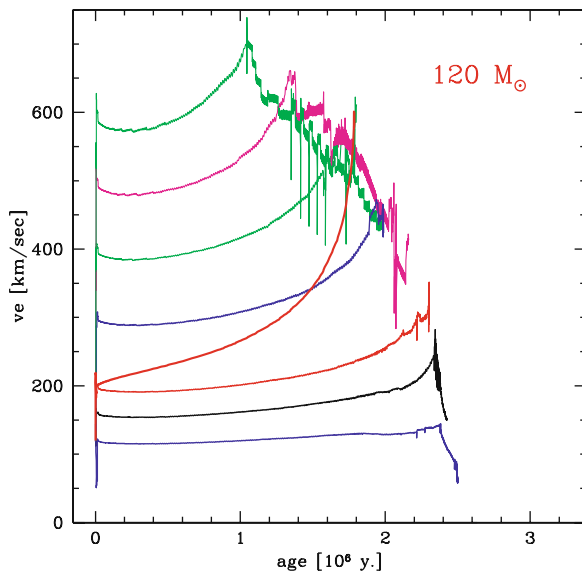
Fig. 27.23 Evolution of the rotational velocities for a 120 M_{\odot} star at Z = 0.02 with different initial rotational velocities v_{\text{ini}} . The right envelope of the curves is the location where the stars reach their critical velocities. A model with solid body rotation with v_{\text{ini}} = 200 \text{ km/s} is also shown, it reaches the critical velocity faster
