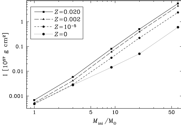
Fig. 13.1 The moment of inertia for stars of various masses and metallicities Z on the zero-age sequence. From S. Ekström et al. [176]
