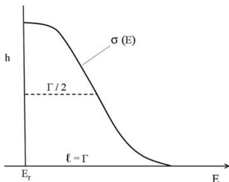
Fig. 9.7 Simplified representation of the resonance
