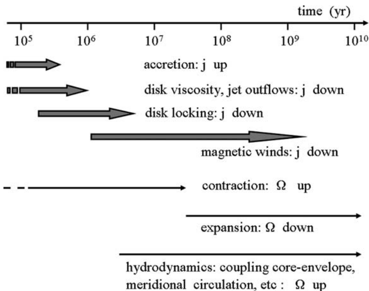
Fig. 21.1 Various effects influence stellar rotation as a function of time for a 1 M_{\odot} star. The thick arrows show the effects changing the specific stellar angular momentum j , while the thin arrows show the effects conserving the angular momentum, but changing the angular velocity \Omega at the stellar surface. Only two hydrodynamical processes are mentioned. Adapted from R.D. Mathieu [385]
