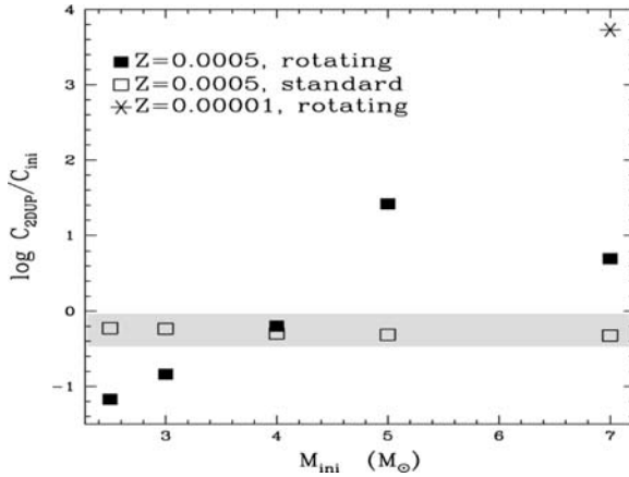
Fig. 26.23 Ratios of the carbon abundance ( ^{12}\text{C} in mass fraction) after the second dredge-up to the initial C content in AGB stars of different initial masses with and without rotation. From T. Decressin and C. Charbonnel [155]
