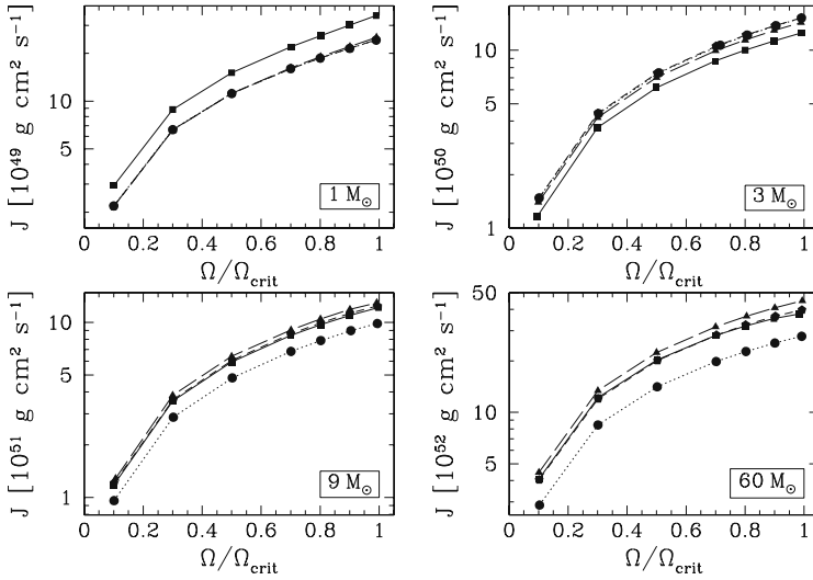
Fig. 13.2 The values of the angular momentum J of stars of different masses on the ZAMS with Z = 0.02 as a function of \omega = \Omega/\Omega_{\text{crit}} . The changes of the stellar radii with rotation are taken into account. Courtesy from S. Ekström
