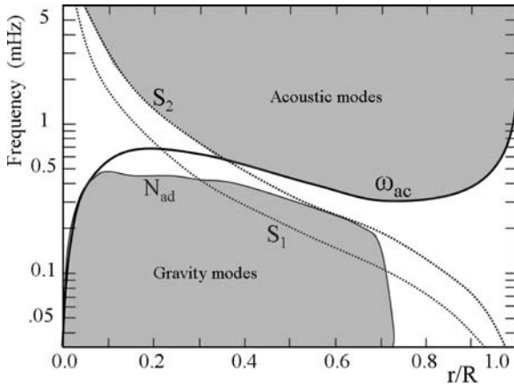
Fig. 16.8 The acoustic cutoff frequency \omega_{ac} is represented by a thick line as a function of the solar radius in the present solar model. The Lamb frequencies for \ell = 1, 2 and the adiabatic Brunt–Väisälä frequency N are also shown. The zone of propagation of g and p modes with \ell = 2 are indicated by gray areas. The zone of p modes is limited near the surface by \omega_{ac} and by the Lamb frequency of the corresponding \ell in the interior (see also Fig. 16.1). For \ell = 1, 2 , the g modes are also limited by S_1 and S_2 . Adapted from P. Eggenberger [169]
