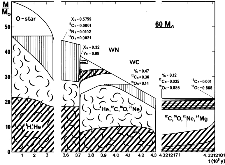
Fig. 27.6 Evolution of the internal structure of a 60 M_{\odot} star ( X = 0.70 , Z = 0.02 ) up to central C exhaustion with mass loss rates [271] and a core overshooting of 0.25 H_p . Values of surface abundances in mass fractions are indicated with an index “s”, while central abundances have an index “c”. WN and WC indicate the Wolf-Rayet stages WN and WC. Same remarks as for Fig. 27.3. From the author [345]
