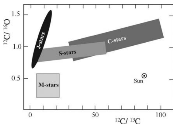
Fig. 26.19 Relation between ^{12}\text{C}/^{16}\text{O} and ^{12}\text{C}/^{13}\text{C} for the different spectral classes of AGB stars. The evolution goes (with shading becoming darker) from M stars \rightarrow S stars \rightarrow C stars \rightarrow J stars. Adapted from V. Smith and D. Lambert [540]; see also M. Forestini [191]
