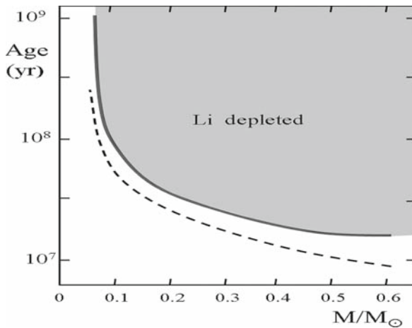
Fig. 20.14 The age of Li depletion as a function of stellar masses. The continuous curve corresponds to a depletion by a factor of 100, the broken line to a depletion by a factor of 2. Adapted from G. Chabrier, I. Baraffe and B. Plez [105]
