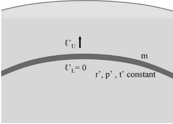
Fig. 15.3 Schematic representation of the one-zone model
