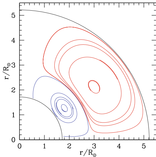
Fig. 11.2 Circulation currents in a 20 M_{\odot} star in the middle of the H-burning phase. The initial rotation velocity is 300 km/s. The inner loop is raising along the polar axis, while the outer loop, the Gratton–Öpik circulation cell, is going up in the equatorial plane. Courtesy by G. Meynet
