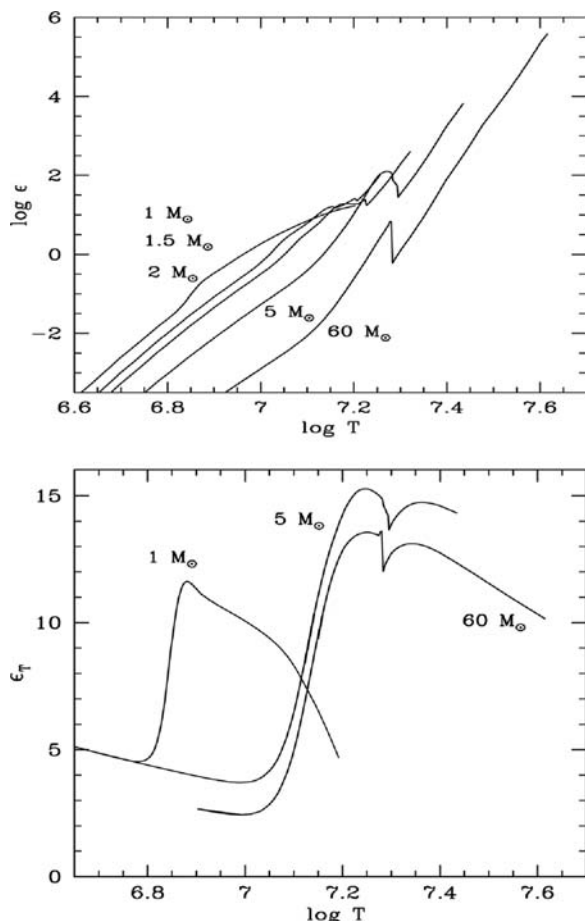
Fig. 25.3 Top : the log of the rates \epsilon of nuclear energy generation in \text{erg g}^{-1} \text{s}^{-1} as a function of T in different stars on the ZAMS and for the present Sun. The kicks in the curves mark the edge of the convective cores. Outside of the cores, the CNO elements are not in equilibrium and this produces higher \epsilon . Bottom : the exponent \nu or \epsilon_T as a function of T
