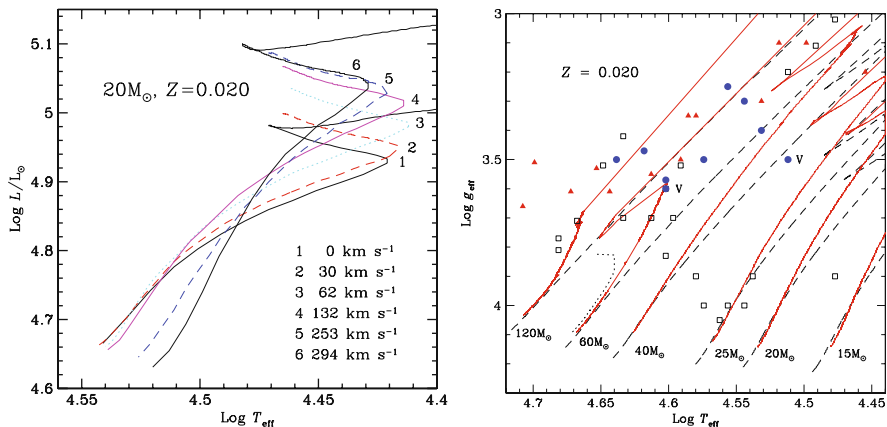
Fig. 27.7 Left : evolutionary tracks of a 20 M_\odot star with Z = 0.02 with different initial velocities. Right : MS tracks in the plot of the effective gravity (including centrifugal force) vs. T_{\text{eff}} . The dashed and continuous lines are for zero rotation and for rotating models with initial v = 300 \text{ km s}^{-1} . Observations by Herrero et al. [245, 246] are shown. From G. Meynet and the author [409]
