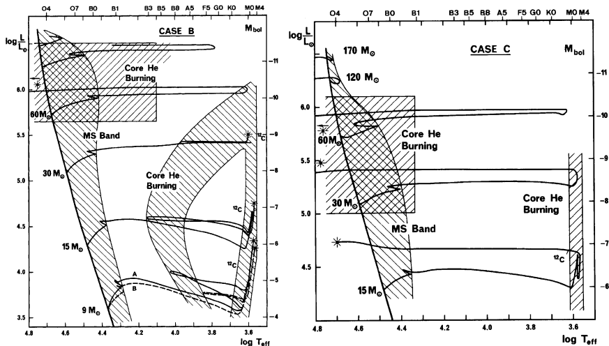
Fig. 27.5 Evolution of massive stars with mass loss and no overshooting for composition X = 0.70 and Z = 0.03 for two cases of mass loss rates with \dot{M} = NL/c^2 (14.1). Left: with N \approx 70 . Right: with N \approx 140 . From the author [339]
