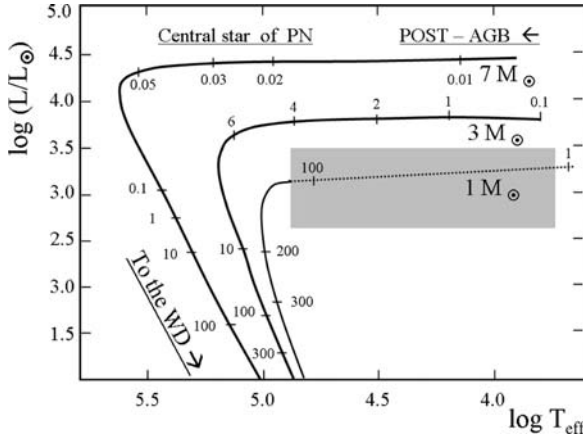
Fig. 26.20 Tracks in the HR diagram for different (initial) masses after the end of the AGB stage. The final masses (WD) are, respectively, 0.94, 0.605 and 0.524 M_{\odot} for 7, 3 and 1 M_{\odot} respectively. The ages after the AGB are given in units of 10^3 yr. The gray area covers several loops of a born-again AGB star resulting from late TP's on the hot side of the HR diagram. Adapted from T. Blöcker [50]
