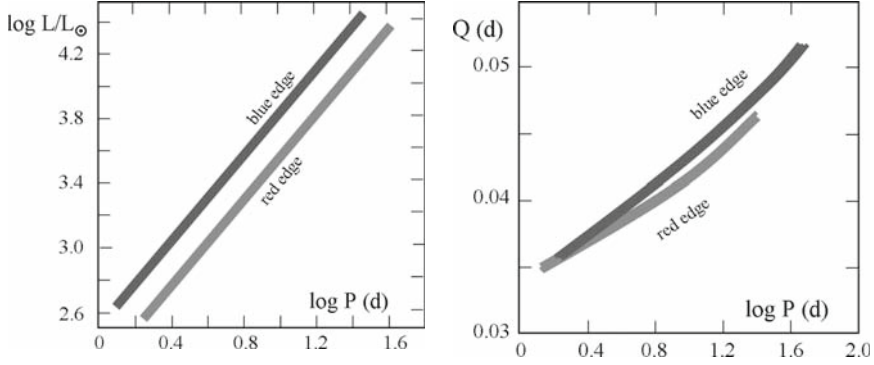
Fig. 15.7 Left : period-luminosity relation for the blue and red edges from numerical models of composition X = 0.70 with Z = 0.02\text{--}0.04 . Right : the pulsation constant Q_0 for the Cepheids as a function of the periods, for the blue and red edge (same symbols as on the left and same composition). Adapted from Saio & Gautschi [504]
