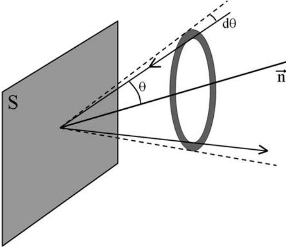
Fig. B.1 Elastic collision of particles with angles between \vartheta and \vartheta + d\vartheta with respect to the normal \mathbf{n} to a surface S
