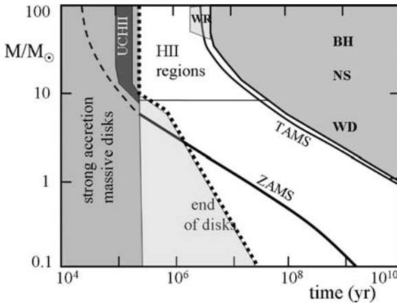
Fig. 18.1 Timescales and properties of stars reaching a final mass M during their formation. The time zero is counted since the formation of a hydrostatic core. Initially, accretion and massive disks maintain the star inside a cocoon. For intermediate masses, the disks survive up to the beginning of the MS phase, while for lower masses the disks disappear before the end of the pre-MS phase. For massive stars, the accretion phase and disks (if any) are present even after the star has reached the ZAMS. TAMS indicates the end of the MS phase, WR means Wolf-Rayet stars. BH, NS and WD mean black holes, neutron stars and white dwarfs. Adapted from Yorke [627]
