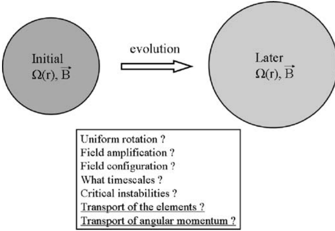
Fig. 13.3 Questions regarding the magnetic field and evolution
