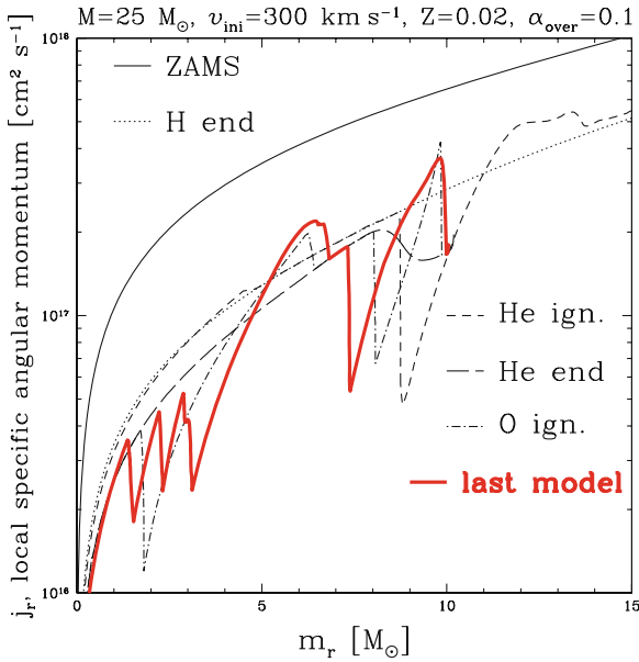
Fig. 28.19 Distribution of the specific angular momentum at various stages for the models of Fig. 28.18. From Hirschi et al. [251]
