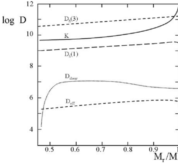
Fig. 12.3 The three diffusion coefficients in the interior of a star model of 20 M_\odot at the beginning of the MS phase. The central H content is X_c = 0.702 , while the initial one was X_c = 0.705 . D_h(2) is almost equal to D_h(3) . K is the thermal diffusivity (3.46). D_{\text{shear}} is the diffusion coefficient by shears (12.68) and D_{\text{eff}} is the diffusion coefficient (11.101) of elements by circulation with account of horizontal turbulence; these two coefficients are calculated here with D_h(3) . From the author [352]
