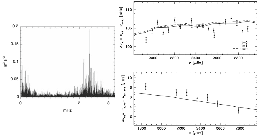
Fig. 16.13 Left : power spectrum of \alpha Cen A, from F. Bouchy and F. Carrier [57]. Right : the large and small separations vs. frequency for \alpha Cen A, comparison of the theoretical curves with the observations indicated by dots with error bars. From P. Eggenberger et al. [171]
