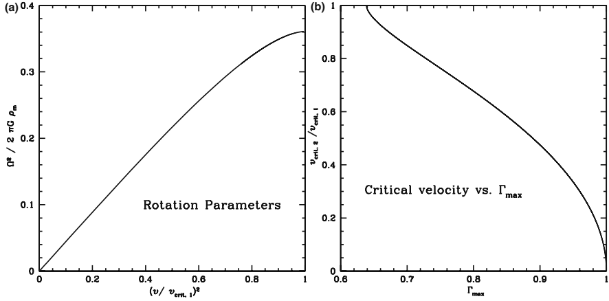
Fig. 4.3 Left: the relation between the rotation parameter \Omega^2/2\pi G\bar{\rho}_M and the ratio of the velocity v to the critical velocity v_{\text{crit},1} . For low enough rotation velocities, one has the relation \Omega^2/2\pi G\bar{\rho}_M \approx \frac{4}{9} \frac{v^2}{v_{\text{crit},1}^2} . Right: the second root or critical velocity v_{\text{crit},2} expressed as a fraction of the usual critical velocity v_{\text{crit},1} as a function of the Eddington factor \Gamma for electron scattering (if the opacity varies over the surface, one has to take the maximum value of \Gamma ). When the Eddington factor tends towards 1.0, the break-up velocity goes to zero
