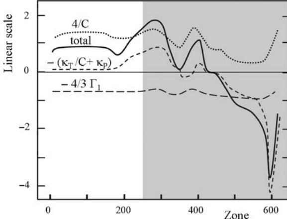
Fig. 15.4 The three terms of condition (15.70) for stability in a Cepheid model of 7 M_{\odot} and their sum. The stellar surface is on the left, the white area is the atmosphere with optical depth < 2/3 , the gray area is the optically thick envelope. Adapted from Schaller [512]
