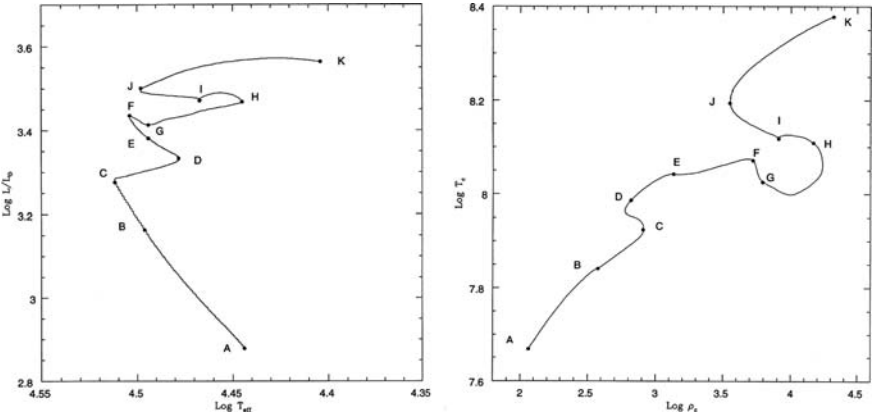
Fig. 29.3 Left: The detailed evolutionary track of a 5 M_{\odot} star at Z = 0 . Further information on the points A, B, C... is given in Table 29.1. Right: central evolution of the same model. From J.M. Feijoo [182]
