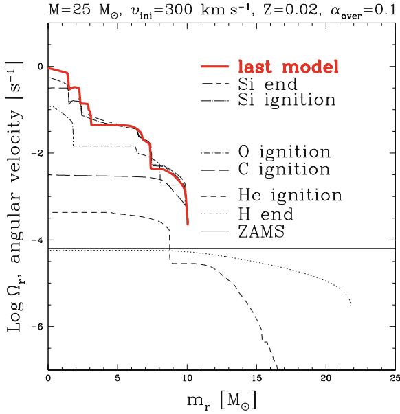
Fig. 28.18 Angular velocity as a function of the Lagrangian mass of a model with initially 25 M_{\odot} , X = 0.705 , Z = 0.02 and v = 300 \text{ km s}^{-1} at various stages up to the collapse (no magnetic fields). From Hirschi et al. [251]
