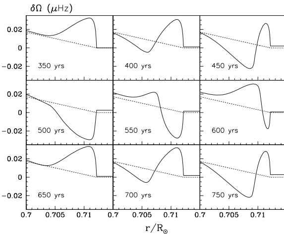
Fig. 17.6 Illustration of the oscillating shear layer (SLO) for a solar model. The lines show the difference of angular velocity with respect to the average in the considered zone at different ages. The dotted line shows the initial \Omega profile. A peak from prograde waves forms first, followed by a negative peak from retrograde waves. The strong shear diffuses first the outer peak then the inner one and the cycles resumes. From S. Talon, P. Kumar and J.P. Zahn [561], with permission
