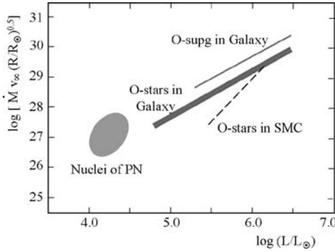
Fig. 14.2 The wind-momentum relation for galactic O stars (class V,III), supergiants and central stars in planetary nebulae (PN), the relation for O stars in the SMC is also shown. Adapted from R.P. Kudritzki and J. Puls [298]
