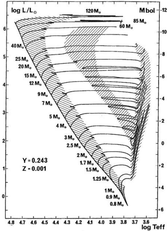
Fig. 26.8 Tracks in the HR diagram of models with composition X = 0.756 and Z = 0.001 . Same remarks as for Fig. 25.17. From [513]
