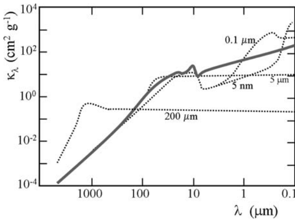
Fig. 22.5 Extinction coefficients for a mixture of dust and gas with a dust-to-gas mass ratio of 0.01. The thick line represents the dust models of Preibisch et al. [478] for dust grains of carbon and ice-coated silicates, which well reproduce the IR and far-IR spectra of protostellar sources. The other lines represent the coefficients for silicate grains of various radii. Grains currently have diameter distributions between 0.005 and 0.25 \mu\text{m} . Adapted from H.W. Yorke [627]
