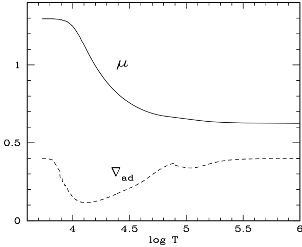
Fig. 7.1 Variations of the mean molecular weight \mu and of the adiabatic gradient (see expression 7.57) as a function of temperature in the outer solar layers
