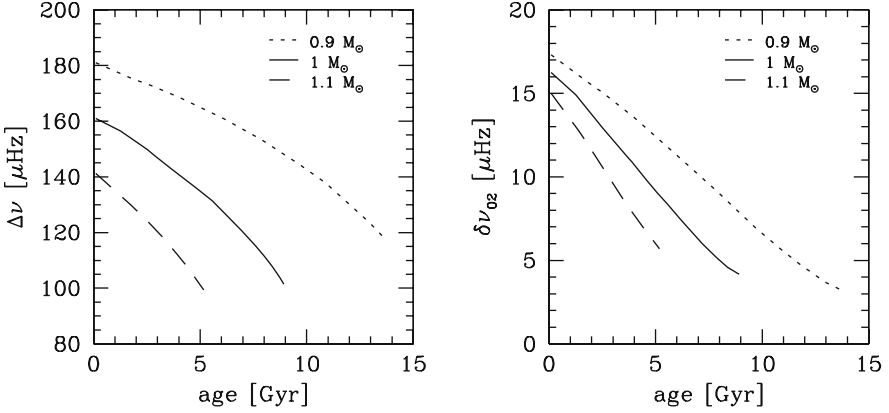
Fig. 16.16 The variations of the mean large and small separations as functions of the ages for different masses. From numerical models by P. Eggenberger [169]
