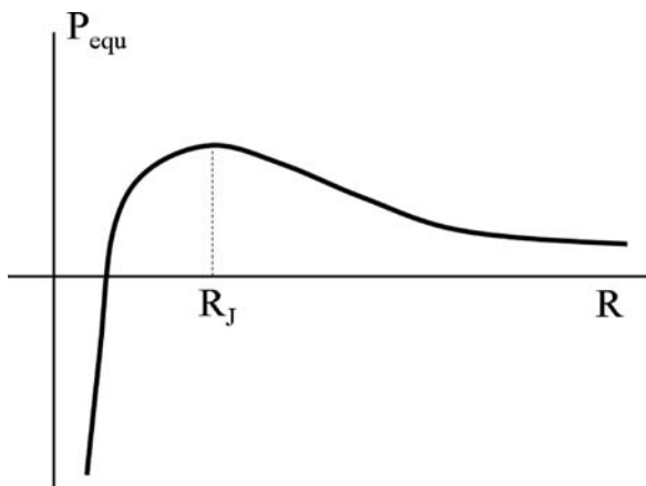
Fig. 18.2 Schematic variation of the equilibrium pressure P_{\text{equ}} as a function of radius R for a spherical body of mass M and temperature T in equilibrium
