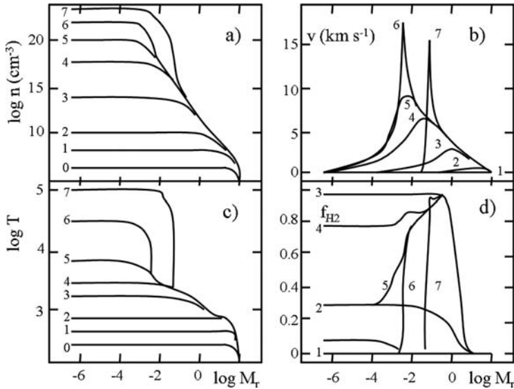
Fig. 23.1 Evolution of the structure of a cloud fragment of 10 M_{\odot} at eight stages of the collapse. The models are labeled from 0 to 7. The panels show (a) the concentration n , (b) the infall velocity, (c) T and (d) the fraction f_{\text{H}_2} of the H nuclei which are inside \text{H}_2 molecules. The horizontal axis expresses the enclosed mass in solar units within the cloud. The age zero is at model 0 with T = 270 K, the age is 720000 yr in model 1, 739000 yr in model 2, 739990 yr in model 3, 739999.6 yr in model 4 where \text{H}_2 is dissociating, then the successive models are within a fraction of year. A core has formed in model 6. Adapted from E. Ripamonti et al. [491]
