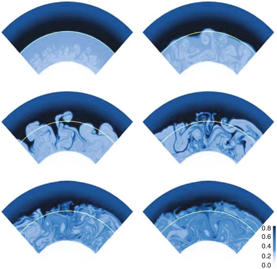
Fig. 6.3 2D numerical simulations of convection in the advanced phase of central O burning. Here, the mixed region ( cloudy ) overshoot by about 30% of the size of the convective region defined by Schwarzschild's criterion ( white curve ). Courtesy from Patrick Young [631]
