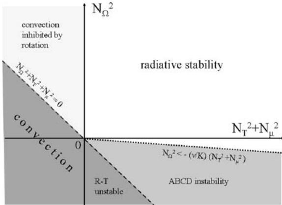
Fig. 12.8 Plot of the instability regions as a function of the Brunt–Väisälä frequency and of the Rayleigh–Taylor frequency N_{\Omega}^2 . According to the Solberg–Høiland criterion (Sect. 6.4.3), for large enough N_{\Omega}^2 convection is inhibited by rotation (6.53). Regions with negative values of N_{\Omega}^2 are Rayleigh–Taylor(R–T) unstable. The ABCD instability develops in the indicated region, the upper limit of which depends on the Prandtl number \nu/K , which is of the order of 10^{-6} . If horizontal turbulence is present, \nu/K may be larger than 1.0
