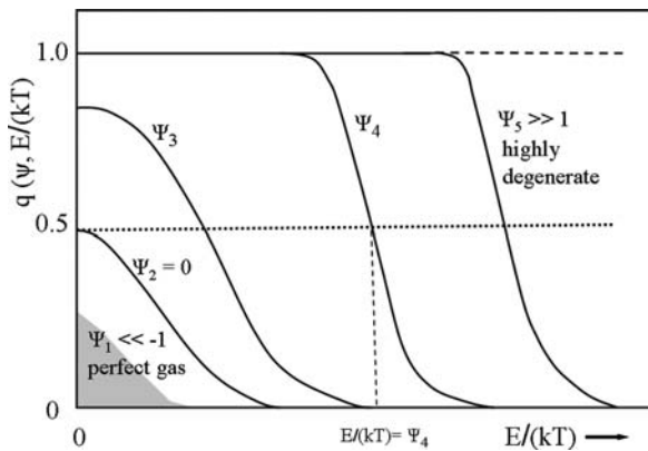
Fig. 7.7 Schematic representation of the occupation factor q(\psi, E/(kT)) as a function of the energy ratio E/(kT) for different values of \psi . The distribution of a perfect gas is shown in grey: degeneracy is increasing from \psi_1 to \psi_5 . The highly degenerate cases tend toward a step function with an edge at the Fermi energy
