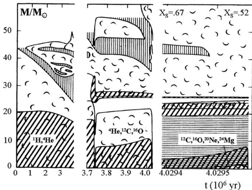
Fig. 27.3 Evolution of the structure (Kippenhahn's diagram) of a star of 60 M_{\odot} with X = 0.70 and Z = 0.03 at constant mass as in Fig. 27.2. No overshooting is included. The H-, He- and C-burning phases are represented with different scales of time. Cloudy regions are convective, heavy diagonal hatching indicates where \epsilon > 10^3 \text{ erg g}^{-1} \text{ s}^{-1} . Vertical hatching indicates variable H and He contents, horizontal hatching indicates variable C and O contents. From the author [338]
