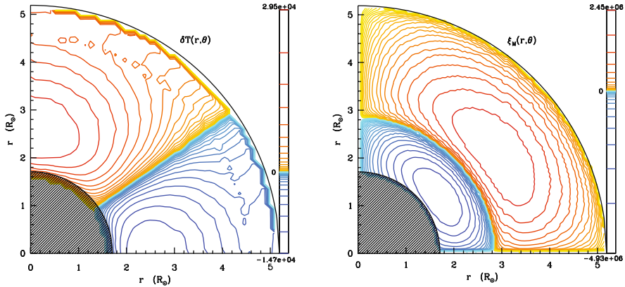
Fig. 11.4 Left : the fluctuations of temperature \tilde{T}P_2(\cos \vartheta) in a rotating 20 M_\odot at the beginning of H burning at an age of 3.5 \times 10^5 yr, as in Fig. 11.3. The initial velocity is 300 \text{ km s}^{-1} , the composition is the standard one with Z = 0.02 . The T excess (up to 2.95 \times 10^4 \text{ K} ) is positive near the polar axis and negative (down to -1.47 \times 10^4 \text{ K} ) close to the equatorial plane. Right : the circulation pattern in the same model, the inner circulation cell is turning clockwise, while the outer one (Gratton–Öpik cell) turns in the opposite direction. Courtesy T. Decressin [153]
