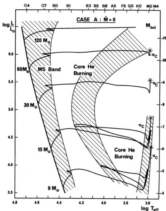
Fig. 27.2 Evolution of massive stars with X = 0.70 and Z = 0.03 at constant mass without overshooting. The hatched areas show the phases of slow H and He burning. The “shiny dots” show the location of the pre-supernovae. The beginning of C burning after He exhaustion is indicated by ^{12}\text{C} . From the author [339]
