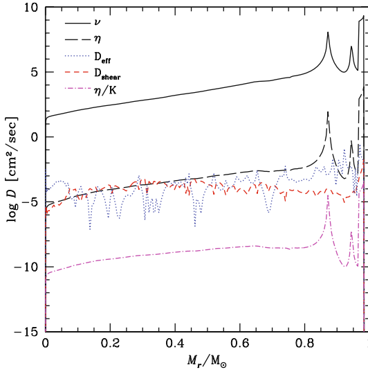
Fig. 13.7 The various diffusion coefficients in a solar model with rotation and magnetic field [172]. \nu expresses the diffusion of angular momentum by magnetic field, \eta the transport of chemical elements by the magnetic instability, D_{\text{eff}} the transport of the elements by meridional circulation, D_{\text{shear}} the transport of the elements and angular momentum by shear turbulence, \eta/K the ratio of magnetic to thermal diffusivity
