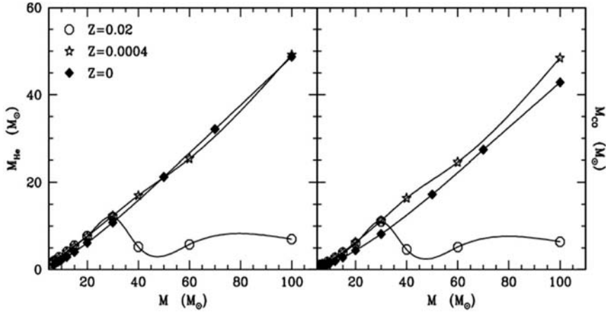
Fig. 29.4 Masses of the He and CO cores at C ignition in models with overshoot and various Z . From P. Marigo, L. Girardi, C. Chiosi and P.R. Wood [377]
