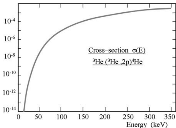
Fig. 9.3 Example of cross-section \sigma(E) in barn ( 10^{-24} \text{ cm}^2 ) as a function of the energy E for the reaction {}^3\text{He}({}^3\text{He}, 2p){}^4\text{He} , the last step of the chain ppI for H burning. This reaction is the main energy source of the Sun. Adapted from Trautvetter [579]
