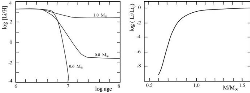
Fig. 20.10 Left : the evolution of the ^7Li abundance as a function of \log (\text{age}) for different masses. The Li abundance is expressed as a number ratio with respect to hydrogen. The value of \log H in the Sun is 12.0. The initial value adopted for the number ratio N(Li)/N(H) is 2 \times 10^{-9} . Adapted from L.T.S. Mendes, F. D’Antona and I. Mazzitelli [397]. Right : the abundance of lithium ^7Li as a function of stellar masses on the ZAMS relatively to the initial abundance Li_0 . Adapted from L. Siess [529]
