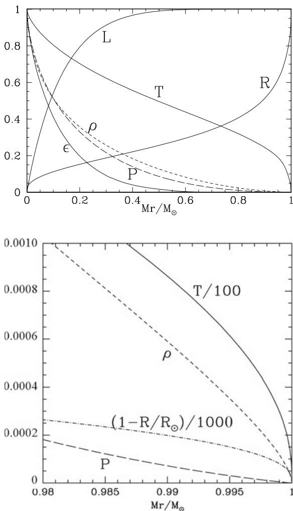
Fig. 25.8 Distribution of luminosity L , temperature T , density \rho , pressure P , energy generation rate \epsilon and radius R as functions of the mass fraction in the present Sun (best fit model for helioseismology). Each variable is normalized to its maximum value, i.e., L = 3.8525 \times 10^{33} \text{ erg g}^{-1} \text{ s}^{-1} , T = 1.5691 \times 10^7 \text{ K} , \rho = 1.5356 \times 10^2 \text{ g cm}^{-3} , P = 2.3453 \times 10^{17} \text{ g cm}^{-1} \text{ s}^{-2} , \epsilon = 1.6982 \times 10 \text{ erg g}^{-1} \text{ s}^{-1} and R = 6.9645 \times 10^{10} \text{ cm} . Bottom figure: details of the outer layers. T is divided by 10^2 . For the radius the quantity (1 - R/R_\odot)/1000 is represented, i.e., a value 0.0002 corresponds to R/R_\odot = 0.80 . Courtesy of P. Eggenberger
