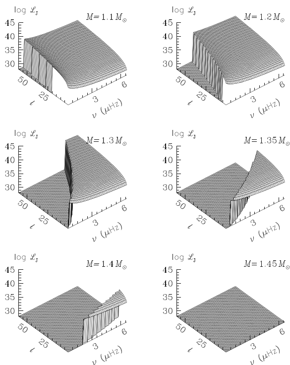
Fig. 17.4 Angular momentum luminosity for stars of various masses for the excitation by overshooting according to R.J. Garcia Lopez and H.K. Spruit [199]. Picture from S. Talon and C. Charbonnel [559]
