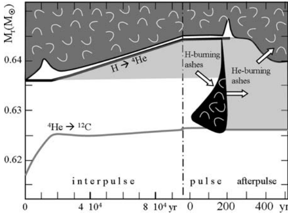
Fig. 26.15 Evolution in an AGB star with an initial 2.5 M_{\odot} . The left side shows an interpulse with H-shell burning. The right side shows the pulse with the He-burning convective tongue. In the afterpulse, dredge-up brings the nucleosynthetic products to the surface as indicated by the arrows . Adapted from N. Mowlavi [434]
