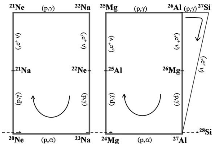
Fig. 25.4 The NeNa (left) and MgAl cycles (right)
