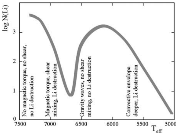
Fig. 17.8 Schematic illustration of the Li dip of the Hyades [52] with the main effects shaping the Li abundances
