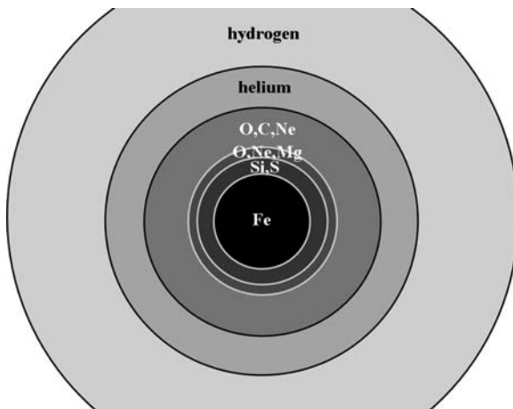
Fig. 28.3 Schematic representation of the onion skin model
