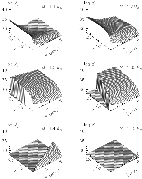
Fig. 17.5 Angular momentum luminosity for various stars with excitation by convective motions [212, 300]. Picture from S. Talon and C. Charbonnel [559]
