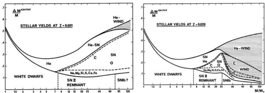
Fig. 28.7 The effects of mass loss on nucleosynthesis, with the mass fractions ejected as a function of the initial mass. The new He, the C, O and heavy elements are indicated, SN means ejected in supernovae. The remnant masses are also indicated in the lower part. The hatched areas indicate the wind contributions in new elements. \dot{M} from de Jager et al. [271], a relation \dot{M} \sim Z^{0.5} is assumed, \dot{M} for WR stars from Langer [306]. Left : low- Z models with small mass loss. Right : models with Z = 0.02 and heavy mass loss. From the author [347]
