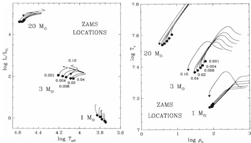
Fig. 26.7 Left : location in the HR diagram of ZAMS models of different Z and Y . Right : values of the central T and \rho for the same models. A relation Y = 0.24 + 2.4Z is adopted. From N. Mowlavi et al. [435]
