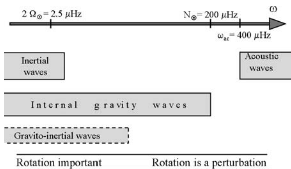
Fig. 17.9 The various types of waves in their frequency domains. The angular velocity, the Brunt-Väisälä frequency and the acoustic cutoff frequency at the base of the convective zone are indicated. Adapted from Mathis [387]
