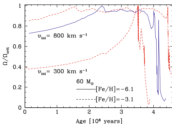
Fig. 29.8 Evolution of \Omega/\Omega_c at the surface of low- Z models of 60 M_{\odot} , with [Fe/H] = -6.1 and -3.1 corresponding to Z \approx 10^{-8} and 10^{-5} , respectively. From G. Meynet, S. Ekström and A. Maeder [407]
