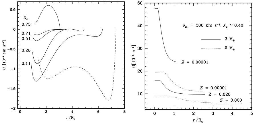
Fig. 11.9 Left: evolution of U_2(r) the radial term of the vertical component of the velocity of meridional circulation for a model of 20 M_\odot with Z = 10^{-5} at various stages during the MS phase (continuous line). X_c is the hydrogen mass fraction at the center. The dashed line shows the values of U(r) inside a 20 M_\odot model at Z = 0.004 when X_c = 0.28 . Right: variation of the angular velocity \Omega as a function of the distance to the center in 3 and 9 M_\odot star models with v_{\text{ini}} = 300 \text{ km s}^{-1} , Z = 0.020 and Z = 10^{-5} and X_c \approx 0.40 . From G. Meynet and the author [410]
