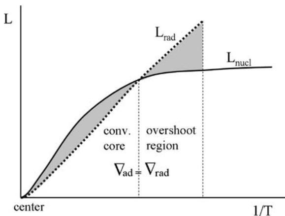
Fig. 6.2 Schematic representation of the Roxburgh criterion for convective overshooting. The various luminosities are represented as a function of 1/T . The Schwarzschild limit is indicated. The overshooting distance is such that the two gray areas are equal. Adapted from [633]
