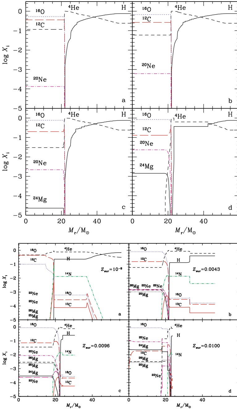
Fig. 29.9 Top : internal distribution of the elements in a 60 M_{\odot} star with Z = 10^{-8} without rotation at the end of He burning. ^{14}\text{N} is below 10^{-8} . Panels a,b,c,d: Y_c = 0.12, 0.06, 0.03, 0.00 with final M = 59.73 M_{\odot} . Bottom : the same for an initial \Omega = 0.73 ( v = 800 \text{ km s}^{-1} ) at similar Y_c . We see the decrease of the total M and the increase of Z at the surface. From G. Meynet, S. Ekström and A. Maeder [407]
