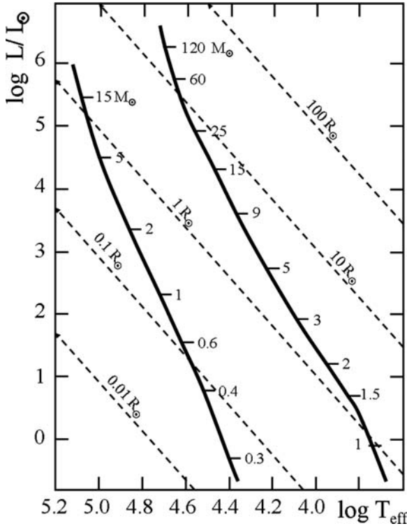
Fig. 24.2 On the right , the zero-age sequences with standard composition X = 0.68 , Z = 0.02 and on the left with helium-rich Y = 0.98 and Z = 0.02 . The masses along the sequences are indicated; the broken lines show loci of constant radii
