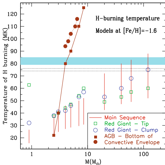
Fig. 26.18 The different T at which H can burn in stars: MS shell H burning, hot bottom burning, etc. The dotted lines show the minimum T for accounting for the observed O, Na, Mg, Al abundances in globular clusters. The thick gray line is the same for H burning in convective zones. Courtesy of C. Charbonnel
