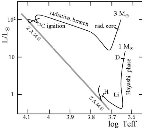
Fig. 20.1 Pre-MS evolutionary tracks for evolution at constant mass for 1.0 and 3.0 M_{\odot} . The places where the ignition of deuterium, lithium and hydrogen starts for the 1 M_{\odot} model are indicated, as well as the ignition of deuterium and ^{12}\text{C} for the 3 M_{\odot} model. Adapted from L. Siess [529]
