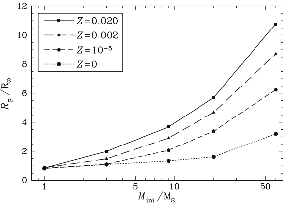
Fig. 25.7 The radii for models on the ZAMS vs. masses for different metallicities Z in the absence of rotation. R_p is here the stellar radius. From S. Ekström et al. [176]
