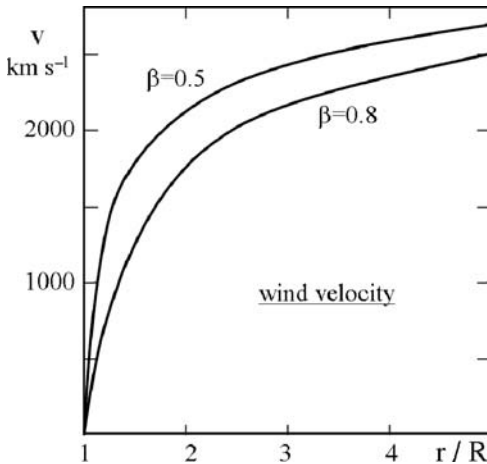
Fig. 14.1 The velocity in the wind as a function of r/R , with R the stellar radius for two cases of \beta in v = v_\infty [1 - (R/r)]^\beta (14.29, see also 14.16). The terminal velocity v_\infty = 3000 \text{ km s}^{-1} in both cases
