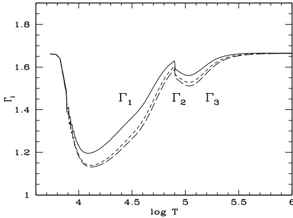
Fig. 7.4 The adiabatic exponents \Gamma_i as functions of temperature in the outer solar layers. In the neutral medium below 8000 K and in the fully ionized medium above T = 3 \times 10^5 K, the various \Gamma_i converge toward 5/3
