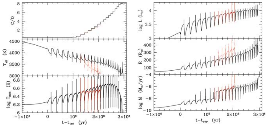
Fig. 26.16 The TP–AGB phase of a 2.5 M_{\odot} star with Z = 0.004 with ( left ) the C/O ratio, T_{\text{eff}} , T at the base of the convective envelope, ( right ) L , R and \dot{M} . The thick continuous lines refer to local opacities corresponding to the local Z , the gray line takes into account of the change of C/O . From T. Decressin [153]
