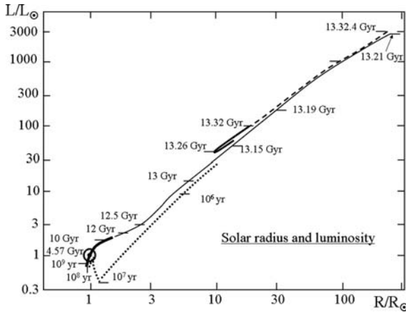
Fig. 25.12 The variations of luminosity and radius of the Sun through the ages. Same source [119] as in Fig. 25.11
