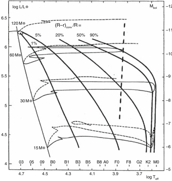
Fig. 5.8 The extent of the external convective envelope of stars in the upper part of the HR diagram, in percents of the stellar radius. Some evolutionary tracks with mass loss ( continuous lines ) and without mass loss ( broken lines ) are indicated. The heavy broken line near \log T_{\text{eff}} = 3.85 is the limit where cooler stars have convective velocities larger than the sound velocity. From the author [337]
