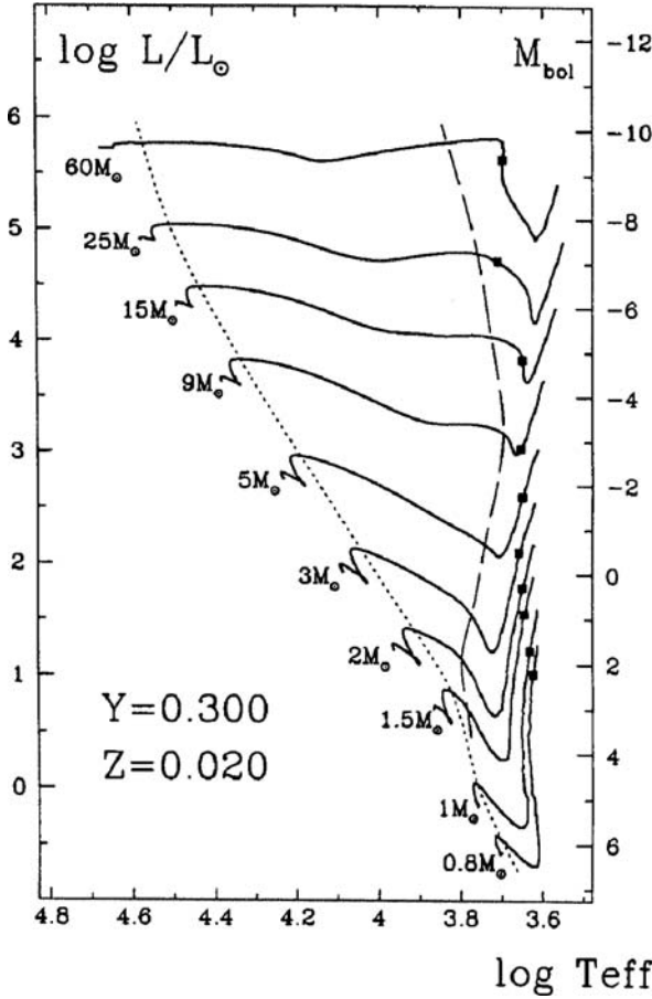
Fig. 20.2 Pre-MS tracks for evolution at constant mass. The squares on the tracks show the location of D ignition. The long-broken line represents the end of the convective envelope, the dotted line the appearance of convective cores (which rapidly disappear for lower masses). From P. Bernasconi and the author [44]
