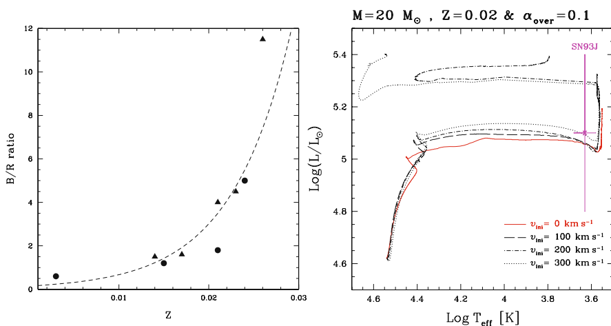
Fig. 27.9 Left : the blue to red-supergiant ratios B/R at different Z in clusters of \log(\text{age}) = 6.8\text{--}7.5 . “B” includes B- and A-type supergiants, “R” the K and M supergiants. From P. Eggenberger et al. [173]. Right : evolutionary tracks for 20 M_{\odot} stars at Z = 0.02 with different initial velocities. From Hirschi et al. [251]
