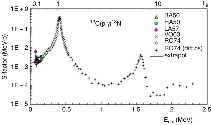
Fig. 9.6 Various empirical determinations of the factor S(E) as a function of energy for the reaction ^{12}\text{C}(p,\gamma)^{13}\text{N} , which is one step of the CN cycle. There are broad resonances. From the Nacre Library, European Compilation of Reaction Rates for Astrophysics, with permission
