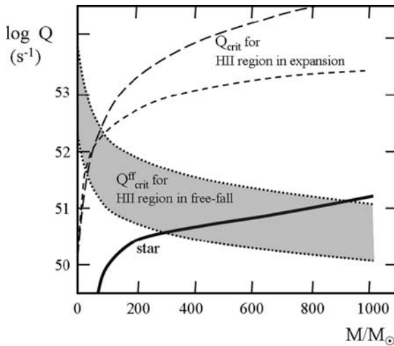
Fig. 23.5 The continuous thick line gives the number of ionizing photons Q emitted by Z = 0 stars as a function of mass. If the number of emitted ionizing photons from a star is higher than Q_{\text{crit}}^{\text{ff}} , an HII region in free-fall grows fast and the high P and T prevent star formation. The lower limit of the gray zone applies to \dot{M}_{\text{accr}} = 10^{-3} M_{\odot} \text{ yr}^{-1} , the upper one to a rate 3.2 times larger. The two upper dashed lines show the limits Q_{\text{crit}} above which an expanding HII region has a photon emissivity which can halt the collapse (Sect. 23.5.3). The upper line ( long dashed ) does not account for the additional effect of electron scattering, while the lower line ( short dashed ) accounts for it. Adapted from K. Omukai and S. Inutsuka [447]
