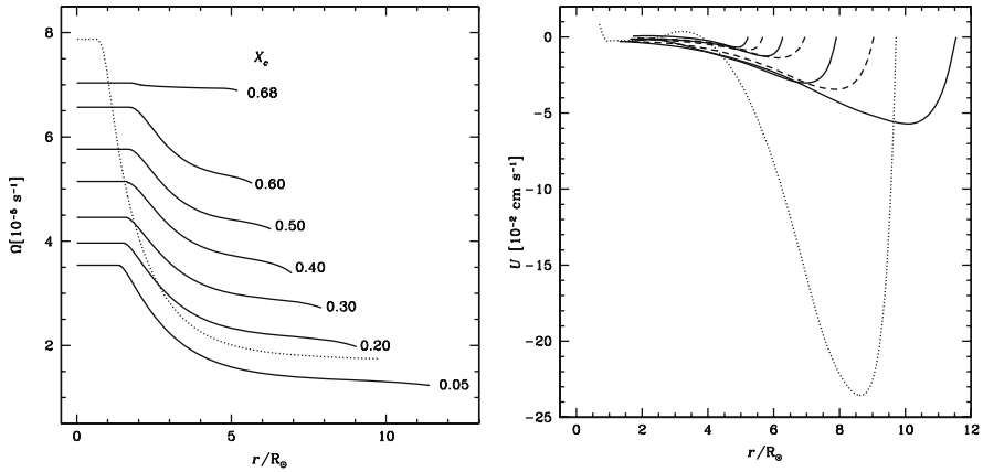
Fig. 11.8 Left : evolution of the angular velocity \Omega as a function of the distance to the center in a 20 M_\odot star with an initial velocity v_{\text{ini}} = 300 \text{ km s}^{-1} and a standard composition with Z = 0.020 . X_c is the hydrogen mass fraction at the center. The dotted line in both figures shows the profile when the He core contracts at the end of the H-burning phase. Right : the vertical component U_2(r) of the velocity of meridional circulation at the same stages of the MS evolution. The negative component becomes more important at the end of the MS due to the decrease of density in the outer layers. From G. Meynet and the author [409]
