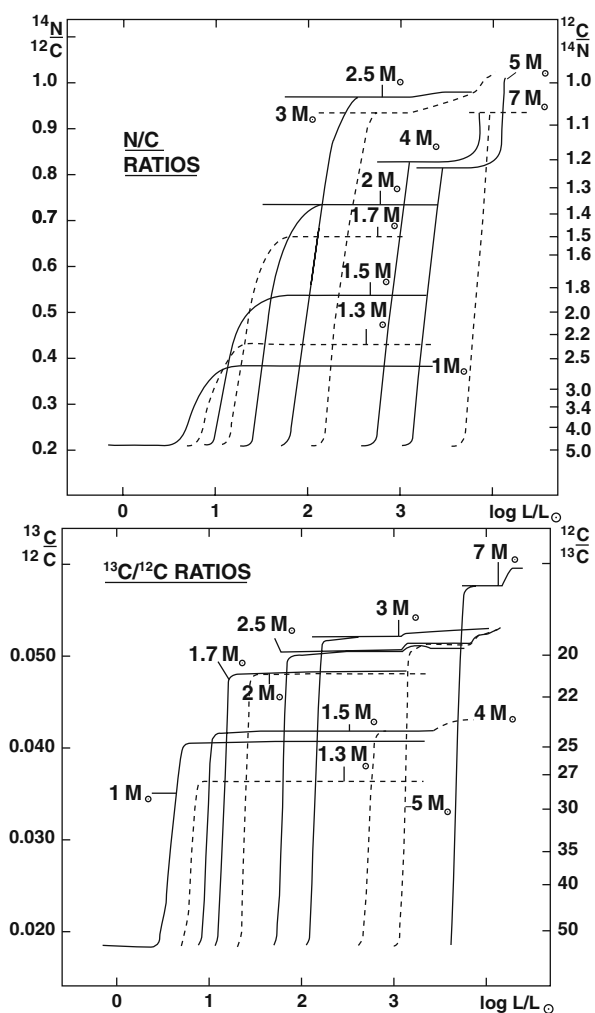
Fig. 26.3 Top : evolution of the surface ratio X(^{14}\text{N})/X(^{12}\text{C}) as a function of the luminosity on the red giant branch for different masses. Bottom : the same for X(^{13}\text{C})/X(^{12}\text{C}) . From the author and G. Meynet [363]
