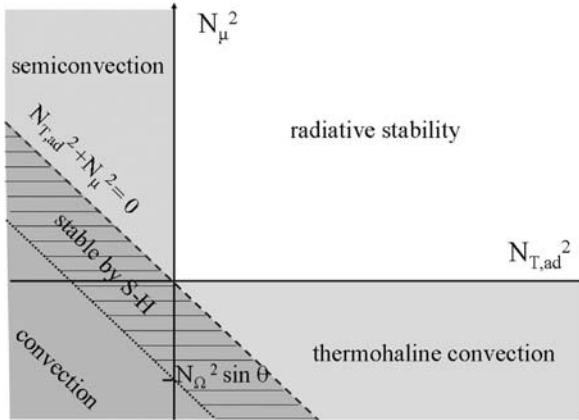
Fig. 6.5 Schematic illustration of the regions of convection, semiconvection, thermohaline convection and radiative stability in the plane showing the thermal and composition terms N_{T,\text{ad}}^2 and N_{\mu}^2 of the Brunt–Väisälä frequency as defined in (5.60). The hatched region schematically indicates where stabilization by rotation may occur due to the Solberg–Hoiland (SH) criterion (see Sect. 6.4.3)
