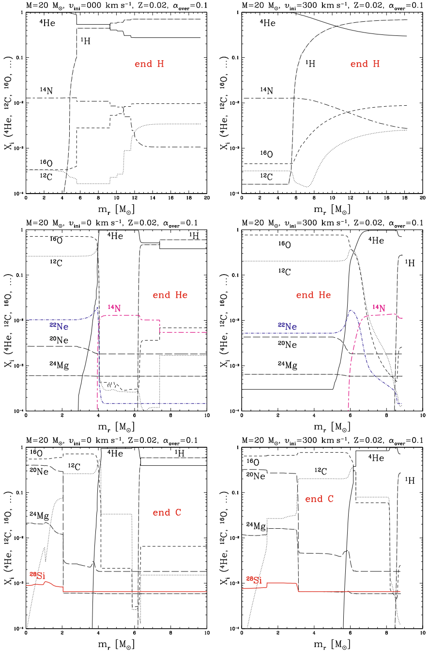
Fig. 28.1 Abundances in mass fraction as a function of mass at the end of central H ( top ), He ( middle ) and C ( bottom ) burnings for non-rotating ( left ) and rotating ( right ) 20 M_{\odot} models with X = 0.705 and Z = 0.02 . From R. Hirschi et al. [251]
