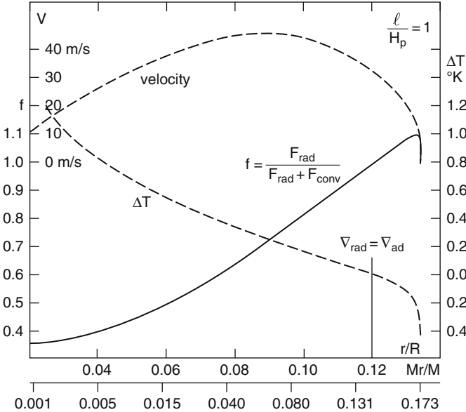
Fig. 6.1 The velocity v , excess \Delta T and ratio f = 1/\mathcal{N}u = F_{\text{rad}}/(F_{\text{rad}} + F_{\text{conv}}) in the convective core of a 2 M_\odot star on the ZAMS. From the author [335]
