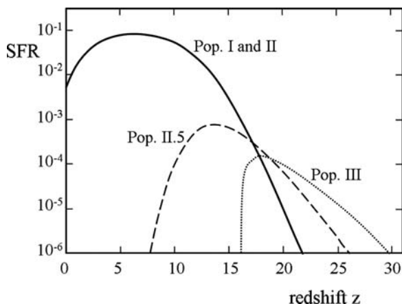
Fig. 23.7 The star formation rate in M_{\odot} \text{ yr}^{-1} \text{ Mpc}^{-3} of Pop. III, Pop. II.5 and Pop. I/II as function of redshift. Adapted from T.H. Greif and V. Bromm [221]
