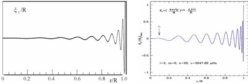
Fig. 16.2 Left : the relative amplitude \xi_r/R as a function of the radius in a solar model, n = 20 and \ell = 2 . The amplitude decreases fast with depth. Right : oscillation amplitude for the case n = 20 and \ell = 2 , but with a normalization by the square root of the inner density. Courtesy of P. Eggenberger [169]
