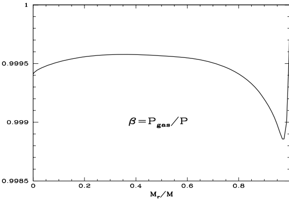
Fig. 3.3 Variation of the ratio \beta of the gas pressure to the total pressure as a function of the mass fraction in the Sun
