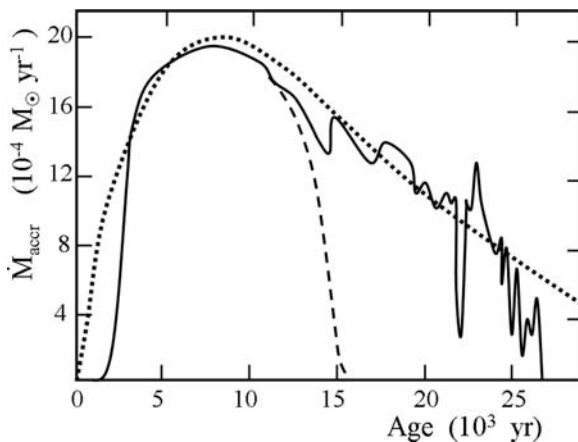
Fig. 22.7 Time evolution of the accretion rate in a model of a cloud clump collapse. The mass of the clump is 60 M_{\odot} and the mass of the star after about 25000 yr is about 33 M_{\odot} . The continuous line refers to a model where a frequency-dependent opacity is considered, while the dashed line shows a gray case. Adapted from H.W. Yorke and S.R. Sonnhalter [630]. The dotted line shows the fitting formula (19.26) of S. Schmeja and S.R. Klessen [518] for \dot{M}_0 = 2 \times 10^{-3} M_{\odot} \text{ yr}^{-1} and \tau_0 = 8000 \text{ yr}
