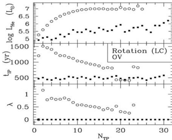
Fig. 26.24 Effects of rotation ( black dots ) on the properties of TP-AGB star of 7 M_{\odot} with Z = 10^{-5} . Local conservation of angular momentum is assumed. Open circles show models with overshooting only. The tip of He luminosity L_{\text{He}} (pulse luminosity), the interpulse duration t_{\text{IP}} and \lambda (26.20) are shown as a function of the pulse number. From T. Decressin and C. Charbonnel [155]
