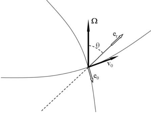
Fig. B.2 The various vectors in the spherical coordinate system
