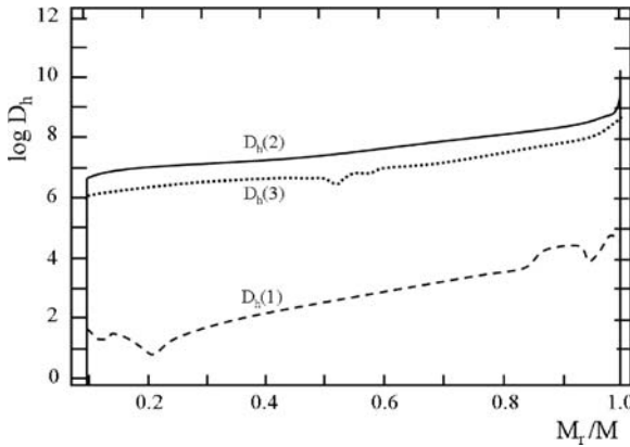
Fig. 12.2 The various coefficients D_h(i) with i = 1, 2, 3 of horizontal turbulence in a 1.5 M_\odot star at an age of 1.368 \times 10^9 yr. A value A = 0.08 is taken in D_h(3) . The initial rotation was 110 \text{ km s}^{-1} . Adapted from Mathis et al. [388]
