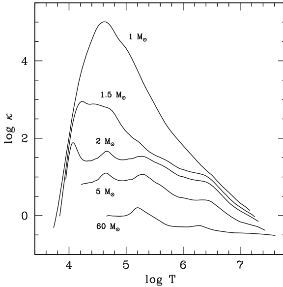
Fig. 8.4 The variation of the opacity as a function of T from surface to center in various stars on the ZAMS, the model of 1 M_{\odot} corresponds to the present Sun
