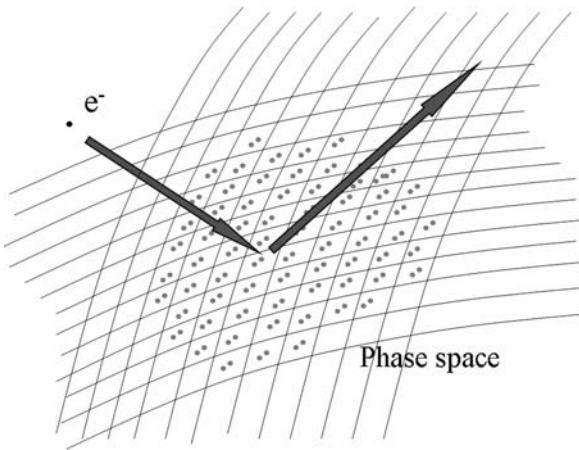
Fig. 7.6 Schematic representation of the phase space of electrons. A new electron is ejected toward cells of higher energy which creates the pressure of degeneracy
