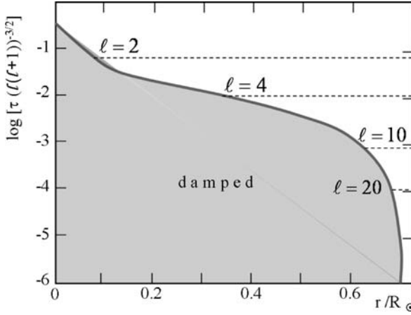
Fig. 17.2 The damping factor divided by (\ell(\ell+1))^{3/2} at \omega = 1 \mu\text{Hz} in the solar model. The depths where this damping term reaches a factor e are indicated. This term is the integral appearing in Eq. (17.39). Adapted from S. Talon [557]
