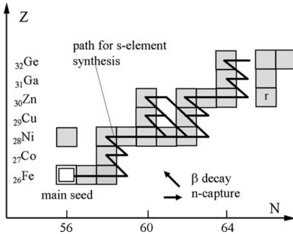
Fig. 28.16 The beginning of the path of s-elements in the Z, N plane of proton vs. neutron numbers. Adapted from F. Käppeler et al. [277]
