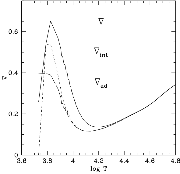
Fig. 5.5 Variations of \nabla , \nabla_{\text{int}} , \nabla_{\text{ad}} in the outer part of the convective envelope of the Sun. \nabla_{\text{rad}} is not represented here, it reaches a peak at 2 \times 10^5 (!) for \log T = 4.6 ; at \log T = 4.8 , it is 9 \times 10^4 and it joins the common curve near \log T = 6.2 . See also Fig. 7.2
