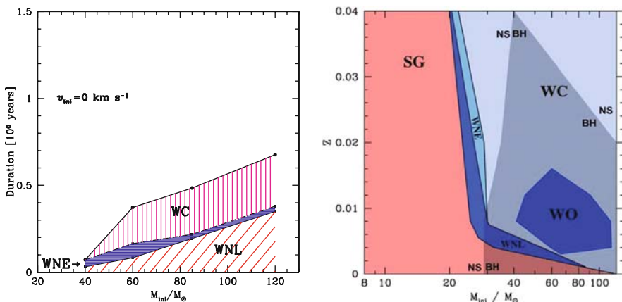
Fig. 27.20 Left: variations of the WR subphases as a function of the initial mass for models without rotation. From G. Meynet and the author [411, 412]. Right: the final stages at the time of the supernova explosion as a function of the initial masses and Z . The final stages as neutron stars (NS) and black holes (BH) are indicated. Courtesy from C. Georgy
