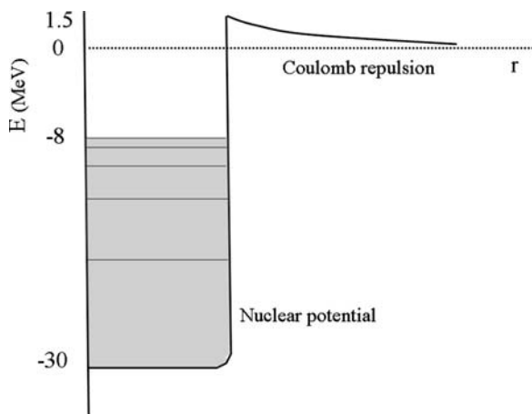
Fig. 9.2 Schematic representation of the nuclear potential well and of the Coulomb barrier in 1/r . The shaded area represents the region occupied by the energy levels of the nucleus. The nucleus is bound with an energy of about -8 MeV. The height of the barrier potential is given by (9.13)
