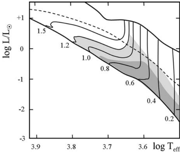
Fig. 20.11 Pre-MS evolutionary tracks for various stellar masses in M_{\odot} . The upper and lower thick lines are, respectively, the birthline and the ZAMS; the broken line is an isochrone of 10^6 yr. In the white area between the two thick lines , there is no Li depletion; in the light shaded area , the depletion is down to 10% of the initial value; in the dark shaded area depletion is between 10% of the initial value and complete depletion. Adapted from S.W. Stahler and F. Palla [548]
