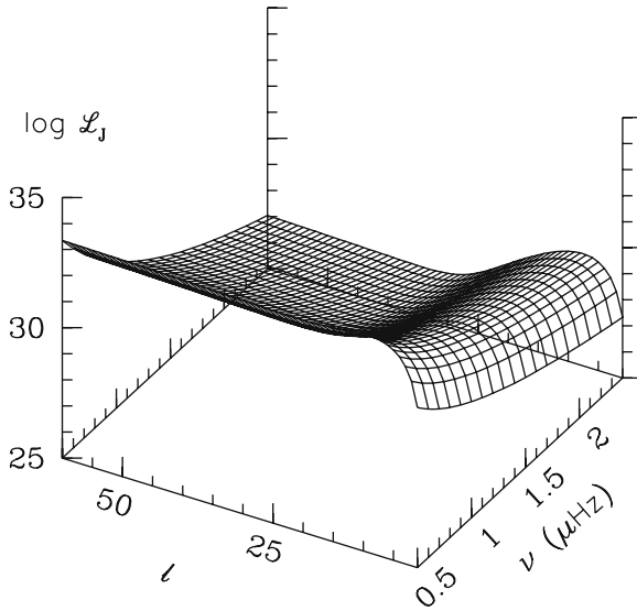
Fig. 17.3 The angular momentum luminosity \mathcal{L}_{\text{ang}} in a 1 M_{\odot} ZAMS model for various degrees \ell as a function of the frequency \nu = \omega/(2\pi) just at the inner edge of the convective envelope. The flux is here calculated with excitation by convective motions (Sect. 17.2.1). Courtesy from S. Talon [557]
