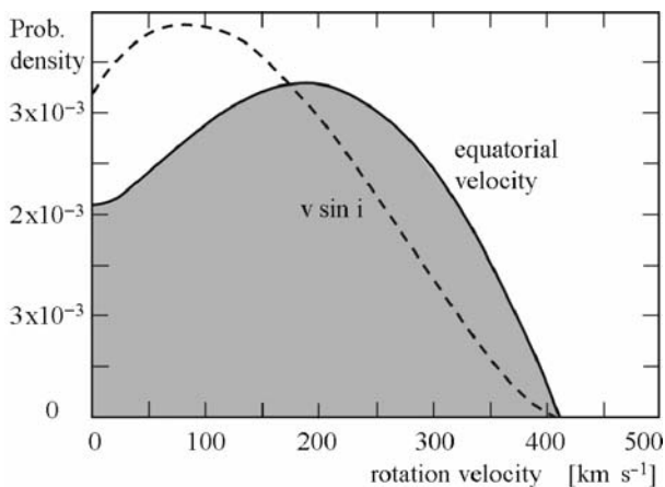
Fig. 27.1 Probability density by \text{km s}^{-1} of rotation velocities for 496 stars with types O9.5 to B8. Adapted from W. Huang and D.R. Gies [256]
