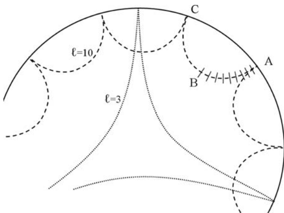
Fig. 16.6 Schematic illustration of mode propagation for \ell = 10 and \ell = 3 . A wave front propagating from A progressively deviates more and more from the radial direction, as the sound speed becomes higher with depth. It reaches its turning point in B before turning back to C. The modes of lower \ell have a deeper turning point for a given oscillation frequency
