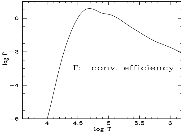
Fig. 5.6 Variation of the convective efficiency \Gamma = \mathcal{P}e/6 in the outer solar layers, calculated with (5.69)
