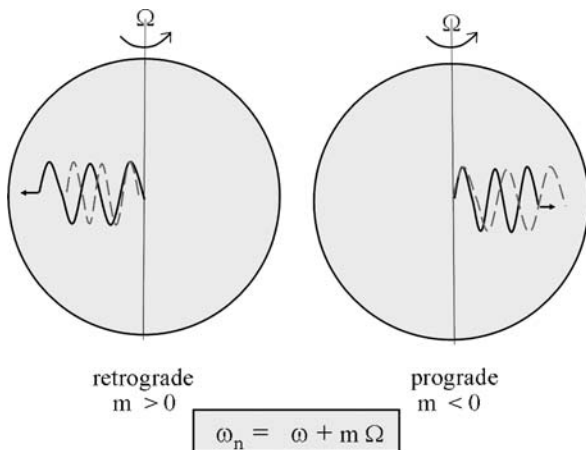
Fig. 16.18 Schematic illustration of retrograde and prograde waves. The wave in the rotating frames are shown in black and the waves as seen by the distant observer are in gray . It looks squeezed in the retrograde case and stretched in the prograde one
