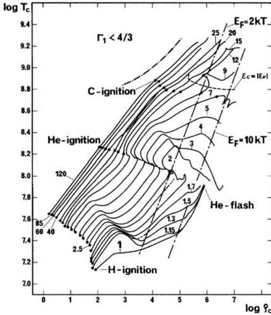
Fig. 26.9 Evolution of the central T and \rho conditions for the models of Fig. 25.17 with an overshooting of 0.25 H_p . The heavy dots indicate the variations nuclear ignitions. The pair instability domain e^+e^- (Sect. 7.8) is indicated by \Gamma_1 < 4/3 . The lines where the Fermi energy E_F of the electrons is equal to 2 and 10 kT are shown. Above the line \epsilon_c = |\epsilon_v| , the neutrino losses are larger than the energy release by C burning. From the author and G. Meynet [363]
