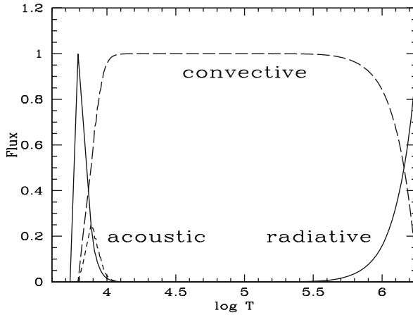
Fig. 5.7 Variation of the fraction of the radiative, convective and acoustic flux with respect to the total energy flux as a function of T in the outer solar layers
