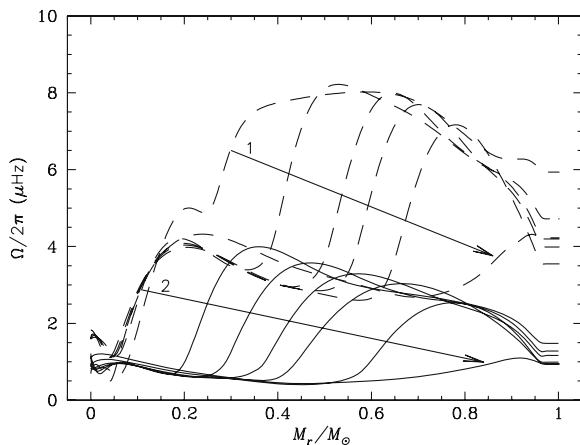
Fig. 17.7 Evolution of the distribution of the angular velocity as a function of time in a 1.0 M_{\odot} model starting from the ZAMS. Account is given to gravity waves, meridional circulation and shear turbulence. The curves with dotted lines (package 1) correspond to ages 0.2, 0.21, 0.22, 0.23, 0.35, 0.27 Gyr, the curves with continuous lines (package 2) correspond to 0.5, 0.7, 1.0, 1.5, 3.0 and 4.6 Gyr. Courtesy from S. Talon and C. Charbonnel [558, 560]
