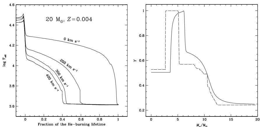
Fig. 27.10 Left: evolution of the T_{\text{eff}} as a fraction of the lifetime spent in the He-burning phase for different initial velocities. Right: distribution of He at the middle of the He-burning phase in a 20 M_{\odot} model at Z = 0.004 with zero rotation ( dashed-dotted line ) and in a model with an initial velocity of 300 \text{ km s}^{-1} ( continuous line ). From the author and G. Meynet [367]
