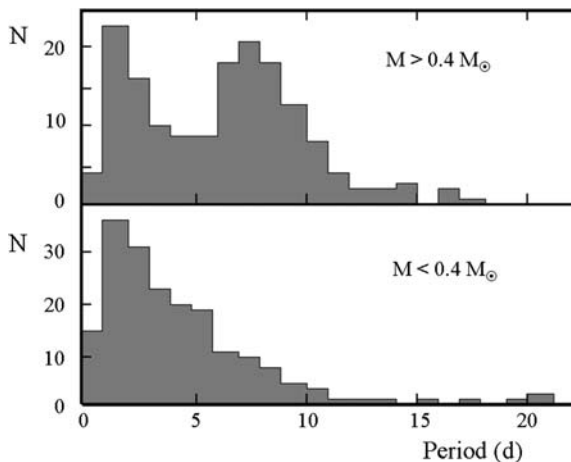
Fig. 21.2 Distribution of the number N of T Tauri stars as a function of the rotation periods for stars in the core of the Orion Nebula. The stars with mass above and below 0.4 M_{\odot} are considered separately. Adapted from R.D. Mathieu [385]
