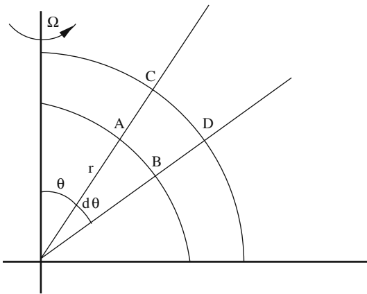
Fig. 10.2 The momentum of the small element ABCD rotating around the vertical axis is derived, r is the radial coordinate of point A and \vartheta its colatitude
