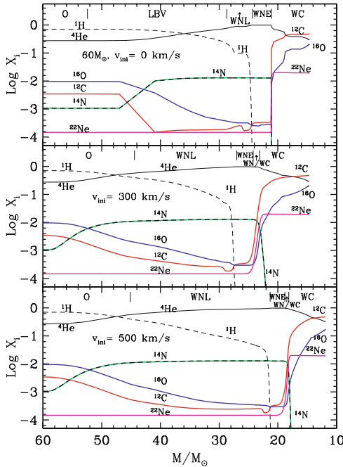
Fig. 27.18 Evolution of the surface abundance for 60 M_{\odot} models at Z = 0.02 for three values of the initial velocities. From G. Meynet and the author [411]
