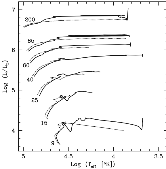
Fig. 29.5 Models with X = 0.76 and Z = 0 up to Si burning (C ignition for 9 and He exhaustion for 200 M_{\odot} ). An overshooting with d_{\text{over}} = 0.2 H_{\text{p}} is applied during the H- and He-burning phases. Models with rotation (continuous lines) and without (dotted lines). From S. Ekström et al. [175]
