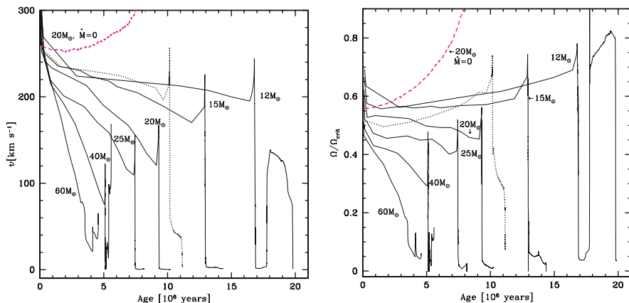
Fig. 27.21 Left: evolution of the rotational velocities as a function of time for the models of Fig. 27.8 with initial velocities of 300 \text{ km s}^{-1} . The dotted line corresponds to a 20 M_{\odot} model with Z = 0.004 . The dashed line applies to a 20 M_{\odot} model at Z = 0.02 without mass loss. Right: the same for the ratio \Omega/\Omega_{\text{crit}} of the angular velocity to the break-up velocity. From G. Meynet and the author [409]
