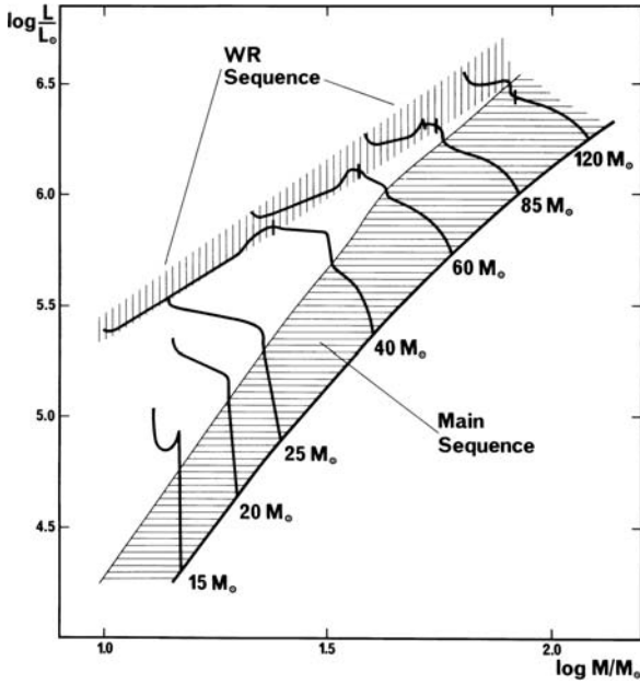
Fig. 27.15 Mass-luminosity relations for MS stars and WR stars ( hatched areas ). The evolutionary tracks are shown, the small slashes on the tracks indicate where the surface H content X_s = 0.3 . From the author and G. Meynet [362]
