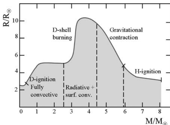
Fig. 20.3 Relation between the radius and mass of a star accreting at a rate \dot{M}_{accr} = 10^{-5} M_{\odot} \text{ yr}^{-1} . Adapted from F. Palla and S.W. Stahler [456, 457]
