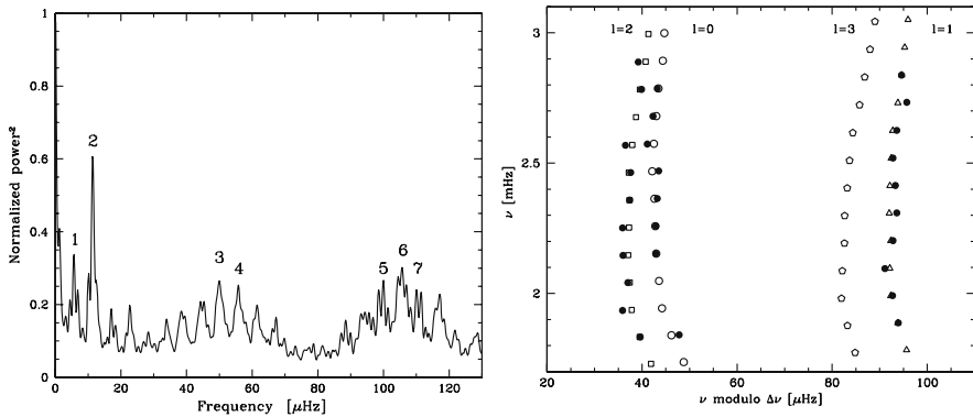
Fig. 16.14 Left : autocorrelation of the power spectrum of \alpha Cen A. Peak nb. 1 at 5.5 \mu\text{Hz} is due to the small separation \delta\nu_{0,2} between modes \ell = 0 and \ell = 2 . Peak 2 at 11.57 \mu\text{Hz} ( = 1/24 \text{ h} ) is the daily alias. Peaks 3 and 4 are due to correlations between modes of \ell = 0, 1, 2 , so that the frequency separation between peaks 3 and 4 corresponds to \delta\nu_{0,2} . Peak 6 at 105.5 \mu\text{Hz} indicates the value of the average separation. Peaks 5 and 7 result from correlations between radial and \ell = 2 modes. The other smaller peaks are due to correlations between modes and daily aliases. From F. Bouchy and F. Carrier [57]. Right : echelle diagram of \alpha Cen A. Open symbols refer to theoretical frequencies; various symbols are used for different \ell , while filled circles give the observed frequencies [57]. From P. Eggenberger et al. [171]
