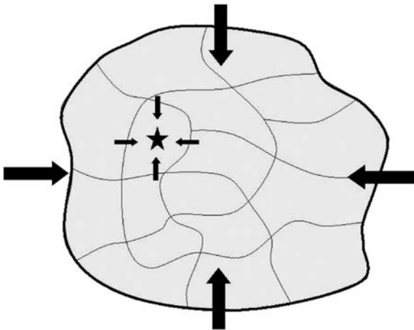
Fig. 18.4 Schematic representation of a cloud contraction and fragmentation
