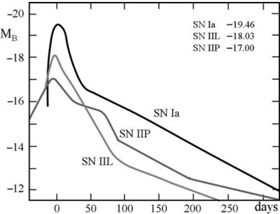
Fig. 28.10 Supernovae lightcurves (days after the maximum). Adapted from K.W. Weiler and R.A. Sramek [609]. The average maxima are from D. Richardson et al. [487]
