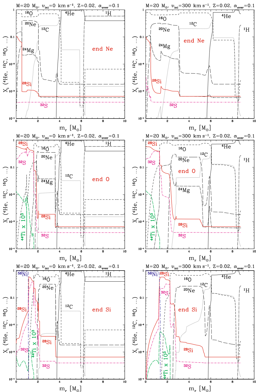
Fig. 28.2 Same as previous figure at the end of central Ne (top), O (middle) and Si (bottom) burnings. The abundance of ^{44}\text{Ti} (dotted-long dashed line) is enhanced by 10^3 for display purposes. From R. Hirschi et al. [251]
