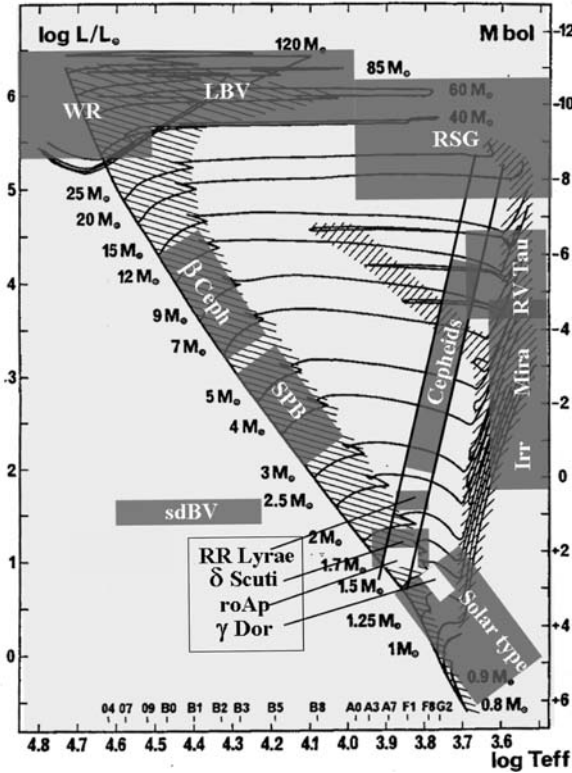
Fig. 15.5 HR diagram with the principal categories of variable stars according to current literature superposed on evolutionary tracks of the Geneva group [513]. These are the Wolf Rayet stars (WR), luminous blue variables (LBV), red supergiants (RSG), \beta Cephei ( \beta Ceph), Cepheids (Cepheids), slowly pulsating B stars (SPB), RV Tauri (RV Tau), Miras, irregular (Irr), blue variable subdwarfs (sdBV), RR Lyrae, \delta Scuti, roAp, \gamma Doradus ( \gamma Dor) and the solar-like stars studied in asteroseismology. The variable white dwarfs are not represented
