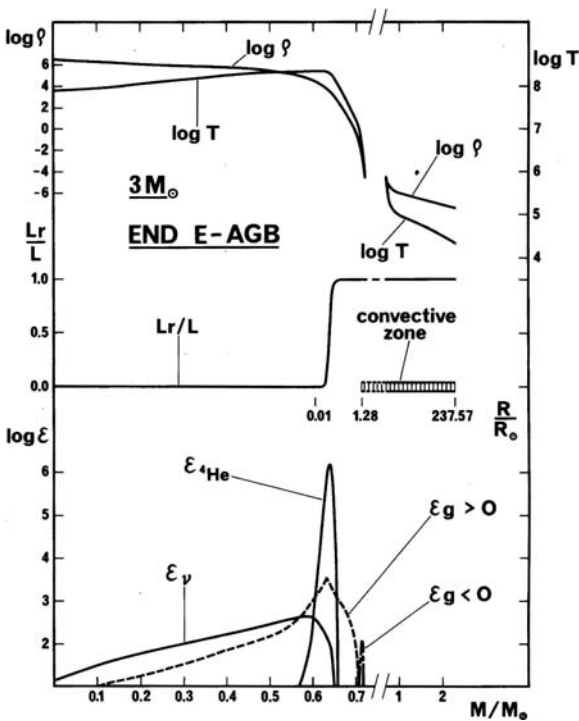
Fig. 26.6 Internal structure, luminosity and various \epsilon rates in a 3 M_{\odot} model at the end of the E-AGB phase. From the author and G. Meynet [363]
