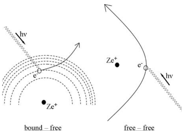
Fig. 8.1 Schematic illustration of the bound–free and free–free absorptions
