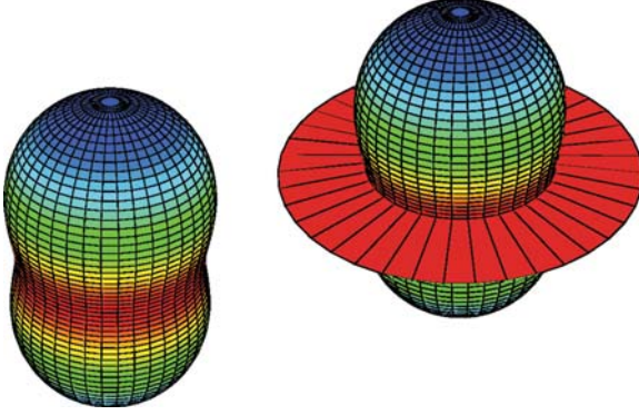
Fig. 14.3 Left : the mass fluxes around a rotating star of 100 M_{\odot} with 10^{6.5} L_{\odot} and a ratio of the angular velocity to the break-up angular velocity \omega = 0.80 , assuming a polar T_{\text{eff}} = 30000 K. Right : the same star but with a polar T_{\text{eff}} = 25000 K; here the opacity jump in the equatorial regions also provokes a ring ejection ( \kappa effect). From the author and V. Desjacques [356]
