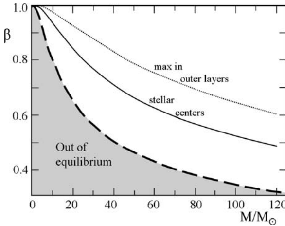
Fig. 3.5 Variation of the ratio \beta = P_{\text{gas}}/P of the gas pressure to the total pressure as a function of the stellar masses on the ZAMS. The continuous line shows the value at the stellar center of models with X = 0.705 and Z = 0.02 , the dotted line gives the maximum value of \beta inside these models. The long-dashed line indicates the minimum value of \beta permitted by relation (3.112) for a value of \mu = 0.618 . Stars in the gray region have too high radiation pressure to be stable
