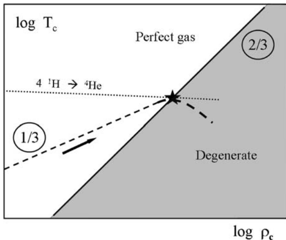
Fig. 3.2 Schematic representation of the central evolution of a star with indication of the perfect gas and degenerate domains separated by a slope of 2/3 (continuous line). The track (dashed line) with an arrow indicates the path with slope 1/3 followed by a contracting star. The dotted line indicates the T limit where H ignition occurs. The star marks the crossing of the dotted and continuous lines, which determines the brown dwarf upper limit
