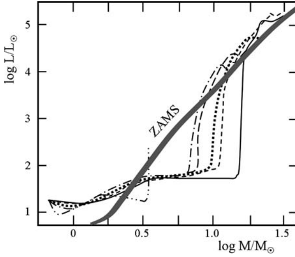
Fig. 22.10 Relation between luminosities and masses for stars on the various birthlines calculated with (19.26). The notation of the lines are the same as in Fig. 22.8. The thick continuous line shows the relation for stars on the ZAMS [464]
