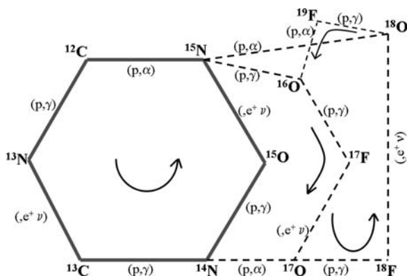
Fig. 25.1 Illustration of CN cycle (hexagon), the two ON loops and an additional branching with indication of the reactions. The whole forms the CNO cycles
