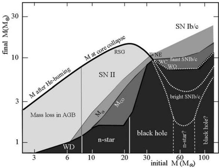
Fig. 28.13 The remnant masses ( black ), the mass of the CO core ( dark gray ), the mass of the He core ( medium gray ), the mass after He burning and at core collapse ( light gray ) as functions of the initial M . The differences with Table 28.3 result from different model assumptions. Adapted from A. Heger et al. [239]
