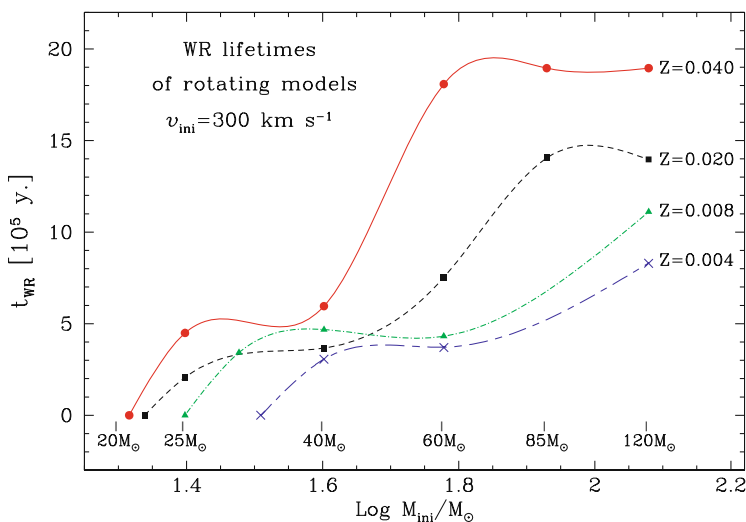
Fig. 27.19 Duration of the WR phases in units of 10^5 yr as a function of the initial masses for models with rotation [412]
