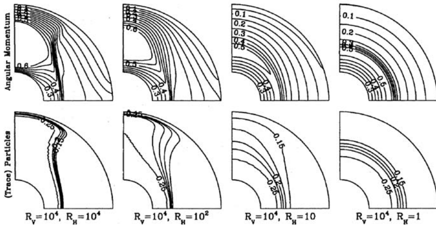
Fig. 12.1 Effects of anisotropy on the distribution of the angular velocity ( top row ) and of the chemical elements ( bottom row ). The various panels show the equilibrium situation for different values of the Reynolds numbers R_H = UR/D_H from 10^4 to 1, where D_H is the coefficient of horizontal turbulence and UR expresses the vertical transport. The vertical Reynolds number R_V = UR/D_V is fixed to 10^4 , where D_V is the vertical diffusion. The two panels show the occurrence of 1D solutions for high horizontal turbulence. From Charbonneau [113]
