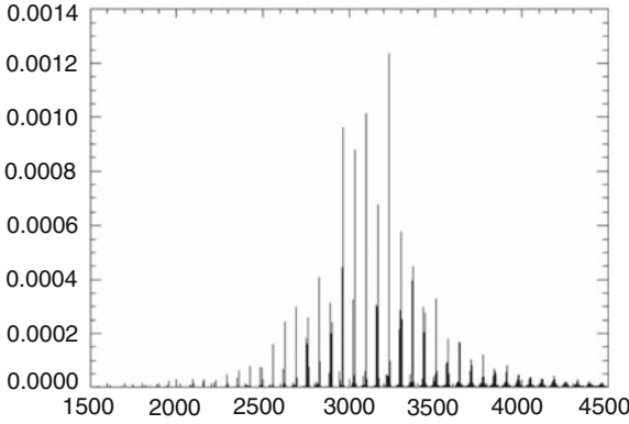
Fig. 16.9 The power spectrum of solar p modes from GOLF on the SOHO satellite (ESA and NASA) with very high signal to noise ratio. The frequency on the horizontal axis is given in \mu\text{Hz} . The vertical scale represents the power in each mode in a linear scale. The doubling of the peaks is generally visible. Courtesy of S. Turck-Chièze
