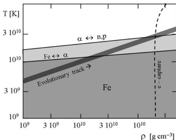
Fig. 28.15 Schematic evolutionary track of massive stars during core collapse with the lines where the half of the ^{56}\text{Fe} nuclei have broken to \alpha and where the half of \alpha have broken to n, p. Adapted from D.N. Schramm [522]
