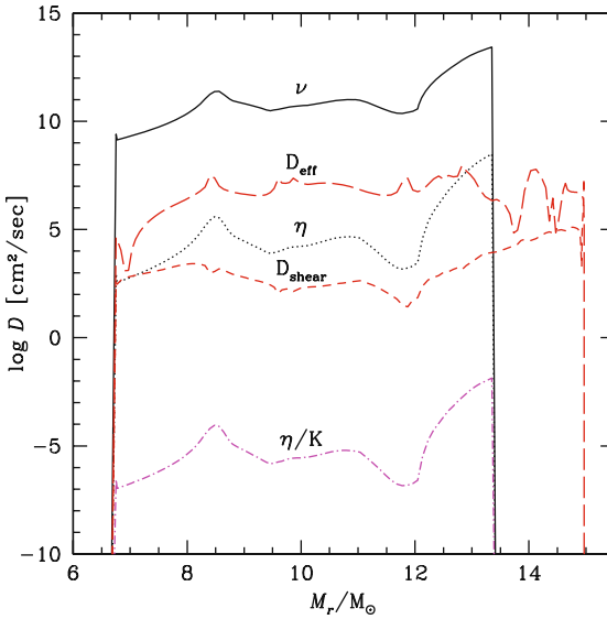
Fig. 13.8 The diffusion coefficients in the model of 15 M_{\odot} with rotation and magnetic field as described in Fig. 13.5. The magnetic field is present in the region where \nu is shown, there B_{\phi} has an average intensity of 2 \times 10^4 G. The various coefficients are defined in Fig. 13.7. From the author and G. Meynet [369]
