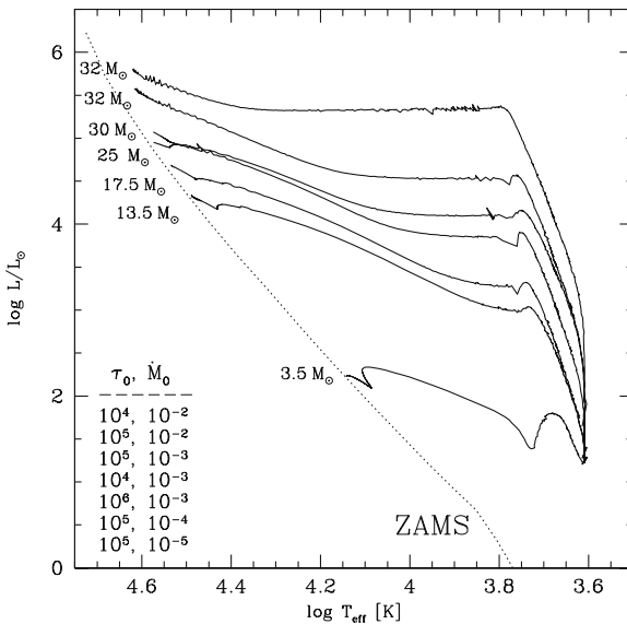
Fig. 22.9 Birthlines calculated with the accretion rates given by (19.26) as in Fig. 22.8. The values of the parameters \tau_0 and \dot{M}_0 are indicated from the top to the bottom. The difference with Fig. 22.8 is that the luminosity here also accounts for the accretion luminosity L_{\text{accr}} . From C. Peter [464]
