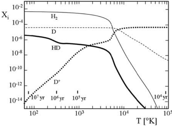
Fig. 23.6 The abundance of HD, H 2 , D and D + as a function of T (with an approximate age scale) in the Z = 0 gas shocked by a supernova at redshift z = 20 (a velocity v = 100 \text{ km s}^{-1} is assumed in the shock, sufficient to produce about complete ionization). Adapted from J.L. Johnson and V. Bromm [275]
