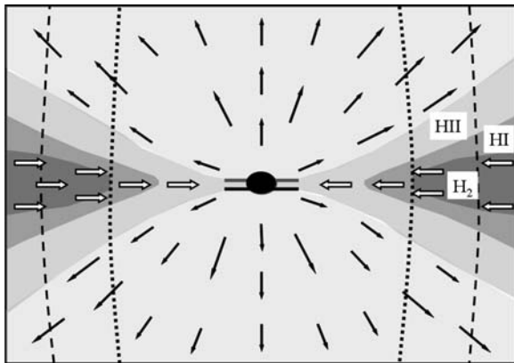
Fig. 22.6 The inner part of the accretion disk, corresponding to the central part of Fig. 22.2. Radiation and bipolar outflows produce evacuated low-density regions symmetrical around the rotation axis (vertical in the figure). These polar cavities are separated from the inner part of the accretion disk by HII and HI regions, with an ionization front at the interface of the two. In the inner part of the disk, molecular gas and dust may survive during the disk lifetime of about 10^5 yr. The dotted line shows r_{\text{sub}} the radius at which dust sublimates; the external broken line shows r_{\text{esc}} the radius beyond which the dust has an escape velocity below 10 \text{ km s}^{-1} , allowing the gas to leave the disk when it photoevaporates. Adapted from H.W. Yorke [627]
