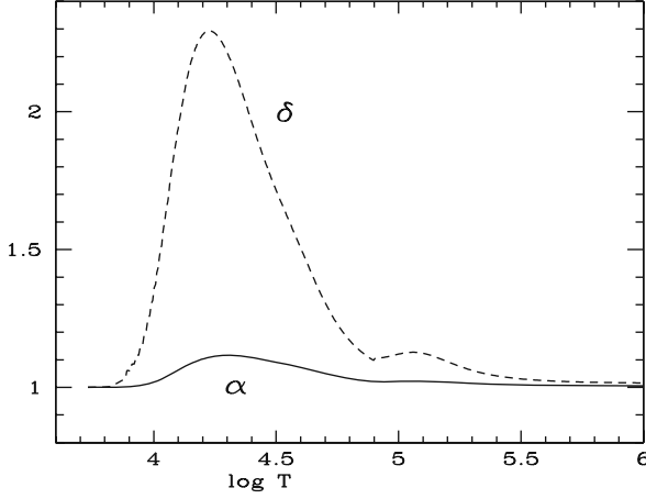
Fig. 7.5 The coefficients \alpha and \delta as a function of T in the outer stellar layers. The variations are due to the change of ionization shown in Fig. 7.2
