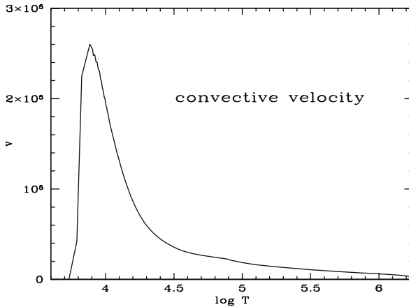
Fig. 5.3 Variation of the average velocity (in \text{cm s}^{-1} ) of convective motions as a function of T in the outer solar layers. The velocity is maximum in the region of partial H ionization, where it reaches up to 30% of the sound velocity. See also Fig. 7.2
