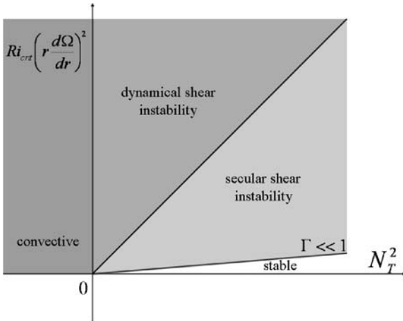
Fig. 12.5 The two terms of the Richardson criterion and the regions of instabilities in the case of medium with constant \mu . In the adiabatic case ( \Gamma = \infty ), when \mathcal{R}i_{\text{crit}} (dV/dz)^2 is larger than N_T^2 , the medium is shear unstable at the dynamical timescale ( middle gray area ). For large thermal diffusivity ( \Gamma \ll 1 ), the instability domain is more extended due to the heat losses which reduce the T stratification ( light gray area ). The limit between the stable and the secular shear instability depends on the value of \Gamma
