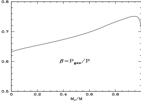
Fig. 3.4 Variation of the ratio \beta of the gas pressure to the total pressure as a function of the mass fraction in a 60 M_{\odot} on the ZAMS
