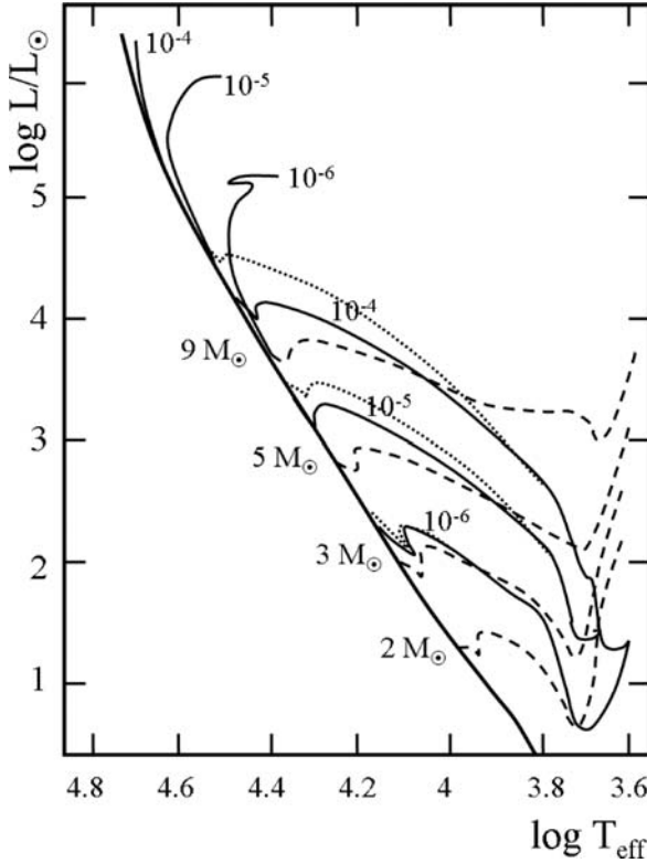
Fig. 20.5 The dashed lines show evolutionary tracks at constant mass (Fig. 20.2). The continuous lines show the birthlines for constant accretion rates \dot{M}_{\text{accr}} = 10^{-6}, 10^{-5}, 10^{-4} \text{ M}_{\odot} \text{ yr}^{-1} ; these birthlines also extend to the upper part of the diagram in the MS stage. The dotted lines represent birthlines for accretion rates slightly growing with mass which may better fit observations for T Tauri stars (cf. Table 20.2; these three dotted birthlines correspond, respectively, to 0.1, 1.0 and 10.0 times the accretion rates considered in Table 20.2 and they start with accretion rates equal to 10^{-6}, 10^{-5} and 10^{-4} \text{ M}_{\odot} \text{ yr}^{-1} , respectively. The thick continuous line is the ZAMS. Adapted from P. Norberg and the author [443]
