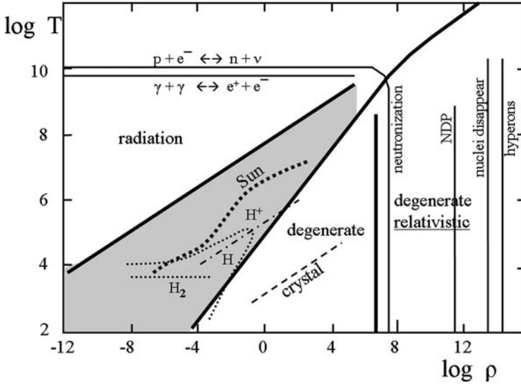
Fig. 7.8 The various domains with different equations of state in the plane \log T vs. \log \rho are schematically shown. In the central gray domain, the law of perfect gas is dominating. The solar model lies in this area ( heavy dots ). The limits for ionized, neutral and molecular hydrogen are shown ( small dots ). The limits between the zones where the radiation pressure, perfect gas pressure, degenerate non-relativistic and degenerate relativistic pressures dominate are indicated by thick lines. The dot-dashed line is the locus where thermal and electrostatic pressure are equal (7.112). A limit for crystallization is shown by a thin dashed line (7.120)
