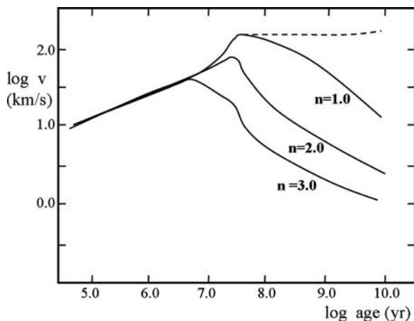
Fig. 21.4 Evolution of the rotational velocity as a function of time for a 1 M_{\odot} star under the assumption of solid body rotation. Various values of n are considered. The pre-MS phase extends up to about 10^7 yr. The broken line shows the evolution without any loss of angular momentum. Adapted from S.D. Kawaler [279]
