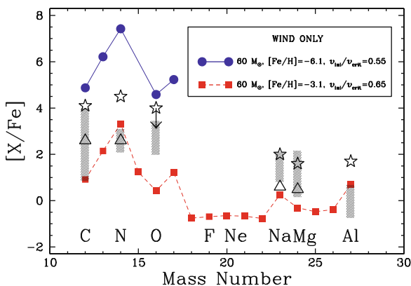
Fig. 29.10 Chemical composition X_i/X(\text{Fe}) (in log scale) of the winds of 60 M_{\odot} models (solid circles and squares) with different compositions ( Z = 10^{-8} and 10^{-5} ) and rotation velocities. The values are normalized to the solar values, e.g., [X_i/X(\text{Fe})]=0 corresponds to the solar abundance ratio for element “i”. The hatched areas, the stars and triangles represent various observations of C-rich very metal-deficient halo stars. From G. Meynet, S. Ekström and A. Maeder [407]
