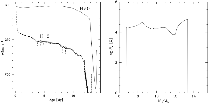
Fig. 13.6 Left : evolution of the equatorial velocity for models of a 15 M_{\odot} with rotation only ( lower curve ) and for the model with rotation and magnetic field ( upper curve ). Same composition and initial velocity as in Fig. 13.5. Right : distribution of the azimuthal component of the magnetic field in the 15 M_{\odot} when the central H content is X_c = 0.60 . From the author and G. Meynet [369]
