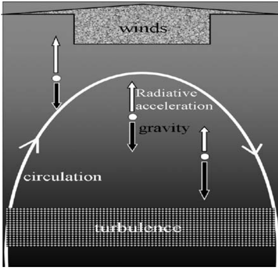
Fig. 10.1 The atomic diffusion results from the balance between the two following main forces: the ions are pushed upward by a radiative acceleration and downward by gravity. These two effects compete with each other. If hydrodynamical processes, such as convection, circulation and turbulence, are present, they are generally largely dominating over atomic diffusion. Adapted from G. Alecian [6]
