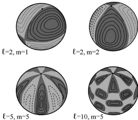
Fig. 16.4 Schematic illustration of some acoustic modes of different spherical harmonic degrees \ell and azimuthal numbers m . Number \ell gives the number of nodal lines (places where v = 0 ) and m the number of nodal lines crossing the equator. The darker areas moves upward while the clearer ones moves downward. The black dots show the point where the rotation axis crosses the surface
