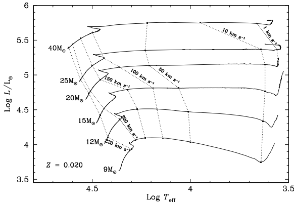
Fig. 27.22 Evolution of the rotational velocities along the evolutionary tracks up to the red giants or supergiants of Fig. 27.8 for initial velocities of 300 \text{ km s}^{-1} . From G. Meynet and the author [409]
