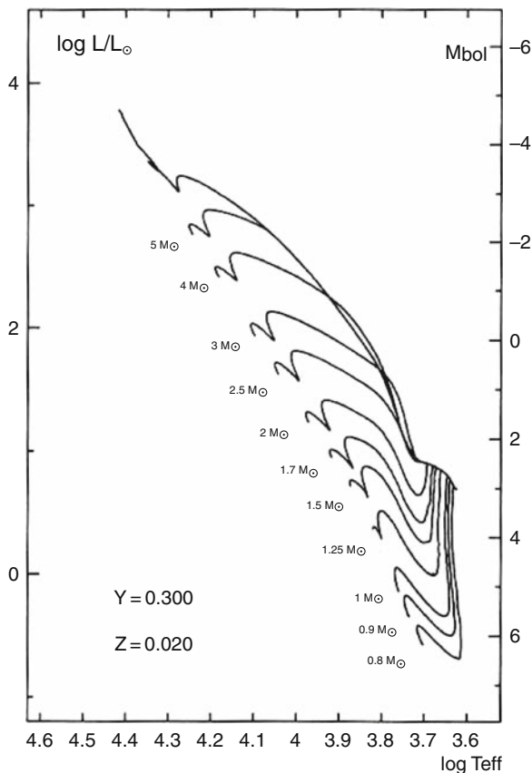
Fig. 20.8 Pre-MS tracks at solar composition with accretion from a cloud with thermal and turbulent support (cf. Table 20.2). The stellar masses on the ZAMS are indicated. The birth-line is indicated by a thick line which forms the upper envelope of the various tracks. From Bernasconi [43]
