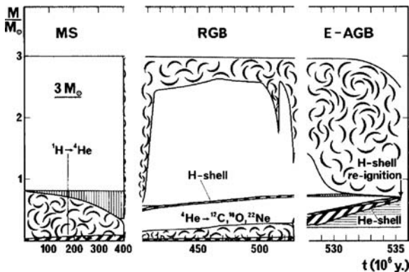
Fig. 26.2 Evolution of the inner structure for a star of 3 M_{\odot} , same remarks as for Fig. 26.1. From the author and G. Meynet [363]
