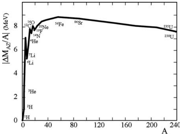
Fig. 9.1 Schematic illustration of the average binding energy |\Delta M_{AZ}/A| per nucleon as a function of the atomic mass number A
