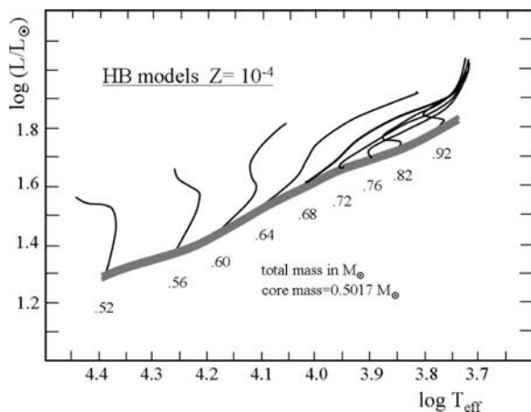
Fig. 26.11 Evolutionary tracks for horizontal branch stars with initial helium content Y = 0.23 , Z = 0.0001 , core mass 0.5017 M_{\odot} and indicated total masses. Adapted from S. Yi, Y.-W. Lee and P. Demarque [625]
