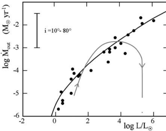
Fig. 22.1 The outflow rates as a function of the bolometric luminosity of the central object (Churchwell-Henning relation). An average inclination angle i = 57.3 degrees is assumed to derive the velocities. The error bar shows the uncertainty for i = 10\text{--}80^\circ . Adapted from Henning et al. [241]. The gray line shows the approximate track for one star described by the expression (19.26) with \dot{M}_0 = 2 \times 10^{-3} M_\odot \text{ yr}^{-1} and \tau_0 = 8000 yr (Sect. 22.4.1)
