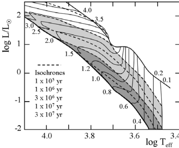
Fig. 20.9 Isochrones of various ages for pre-MS models with constant accretion rates of 10^{-5} M_{\odot} \text{ yr}^{-1} . Light gray shading shows the location of stars between 10^6 and 10^7 yr; dark area is for stars above 10^7 yr. The ages indicated here are t_{\text{pre-MS}} (from the birthline). Adapted from S.W. Stahler and F. Palla [548]
