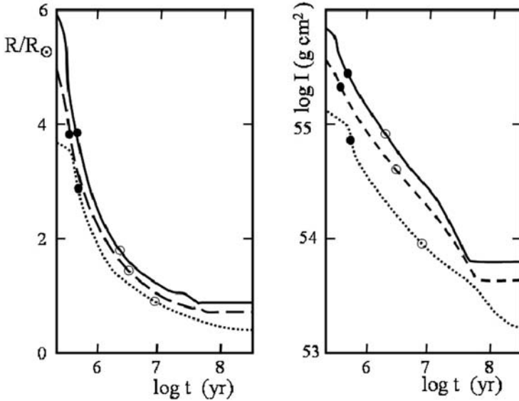
Fig. 21.3 Evolution of the stellar radius R/R_{\odot} (left) and the log of the moment of inertia I (right) for stars of 1 M_{\odot} (continuous line), 0.8 M_{\odot} (broken line) and 0.5 M_{\odot} (dotted line) as a function of age. The black dots indicate the stage at which the star leaves the birthline with \dot{M}_{\text{accr}} = 10^{-5} M_{\odot} \text{ yr}^{-1} . The open dots show the start of a radiative core. Adapted from J. Bouvier et al. [60]
