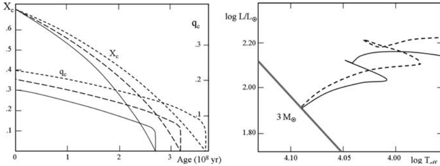
Fig. 25.16 Left: evolution of the core mass fraction for a 3 M_\odot star with the three cases considered in Fig 25.14: no overshooting (continuous line), d_{\text{over}}/H_p \approx 0.08 and twice larger. The evolution of the central H content is also shown. Right: corresponding evolutionary tracks for the cases of no overshooting (continuous line) and of large overshooting. Adapted from the author [336]
