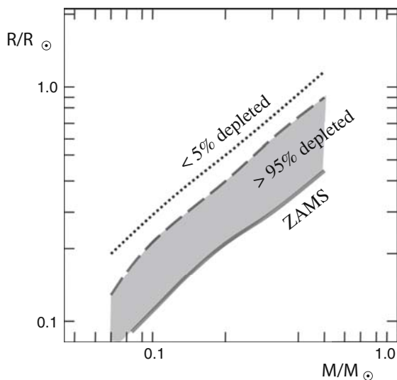
Fig. 20.13 Lines of constant Li depletion as a function of radius and mass. The lines of 5 and 95% depletion are shown. Adapted from L. Bildsten et al. [46]
