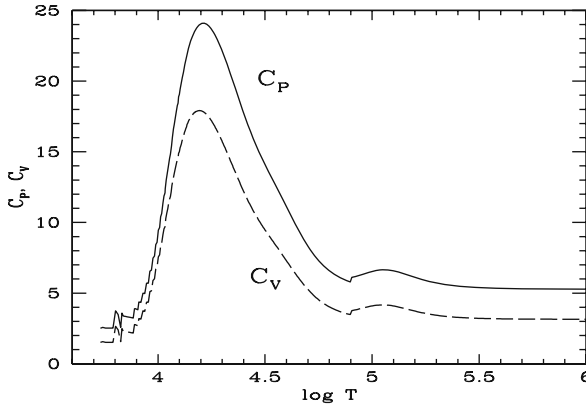
Fig. 7.3 Variations of the specific heats C_p and C_v as a function of T in the outer solar layers. The units of C_p and C_v are \mathcal{R}/\mu_0 . The variations are due to the changes of partial ionization as in Fig. 7.2
