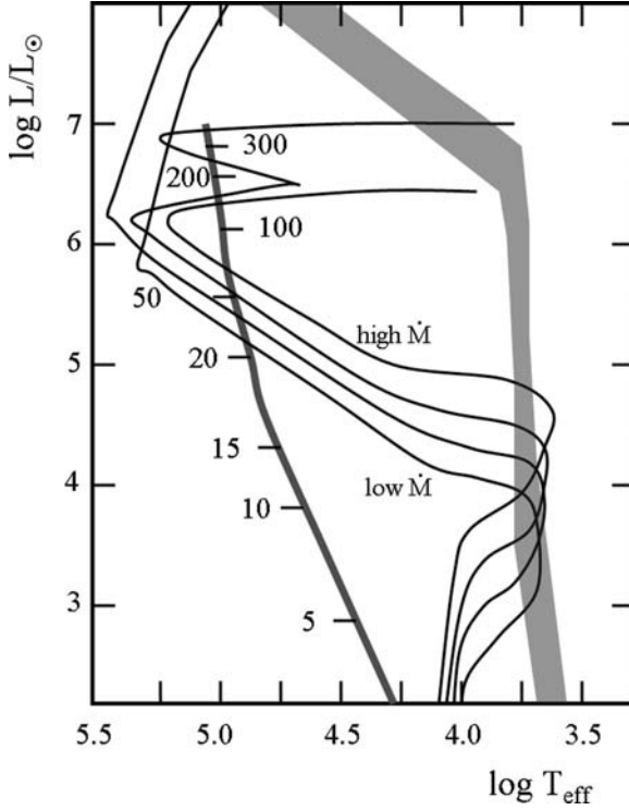
Fig. 23.4 The birthlines of primordial stellar cores for four different accretion rates equal to 1/4 , 1/2 , 1.0 and 2.0 times \dot{M}_{\text{ref}} = 4.4 \times 10^{-3} M_{\odot} \text{ yr}^{-1} . The luminosities are in solar units. The temperatures T_{\text{eff}} are those of the accreting cores. The gray area shows the location of the stars if their photospheric temperature is represented. The ZAMS from non-accreting models is indicated by a thick line with masses in solar units. Adapted from K. Omukai and F. Palla [448]
