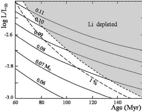
Fig. 20.15 A lithium diagnostic diagram: the evolution of the luminosity of stars near the brown dwarf limit as a function of age. The region where lithium is fully depleted is indicated by a gray area. The locus where lithium is depleted to 1% of the initial level is indicated by a long-broken line . The brown dwarf limit is at about 0.08 M_{\odot} . Adapted from G. Basri, G.W. Marcy and J.R. Graham [37]
