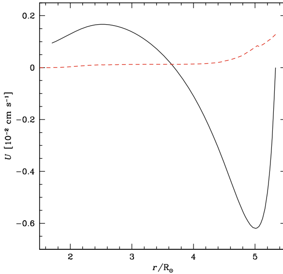
Fig. 11.7 Non-stationary ( continuous line ) and stationary ( broken line ) solutions for U(r) the vertical component of the velocity of the meridional circulation (cf. 11.83) as a function of the distance to the center in a 20 M_{\odot} model at the end of the initial convergence. From Meynet and the author [409]
