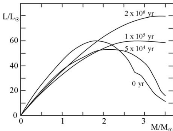
Fig. 20.7 Evolution of the internal luminosity of a 3.5 M_{\odot} star after it has left the birthline. The time is counted since the birthline. There is an outward shift of the luminosity peak as the star tends to thermal equilibrium. During these phases, the surface luminosity grows strongly. Adapted from F. Palla and S.W. Stahler [456]
