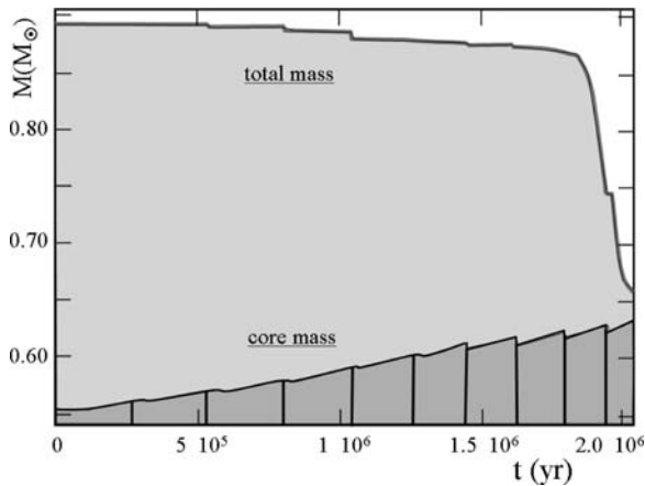
Fig. 26.17 Evolution of the total mass and of the core mass of a 0.9 M_{\odot} with Z = 5 \times 10^{-4} . The mass loss rates are a few 10^{-9} M_{\odot} \text{ yr}^{-1} for the first pulses and reach a few 10^{-5} M_{\odot} \text{ yr}^{-1} in the last two pulses leading to a planetary nebulae. Adapted from M. Forestini [191]
