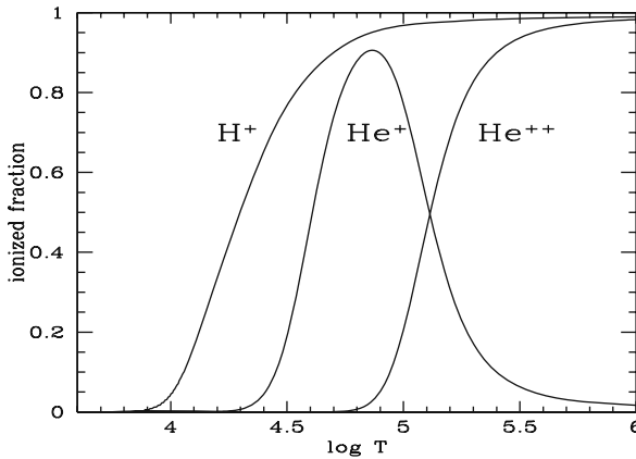
Fig. 7.2 Fractions of ionized hydrogen \text{H}^+ and of ionized helium \text{He}^+ and \text{He}^{++} as a function of the temperature in the outer solar layers of a solar model. T = 10^6 K at M_r/M_\odot = 0.995 , R/R_\odot = 0.846
