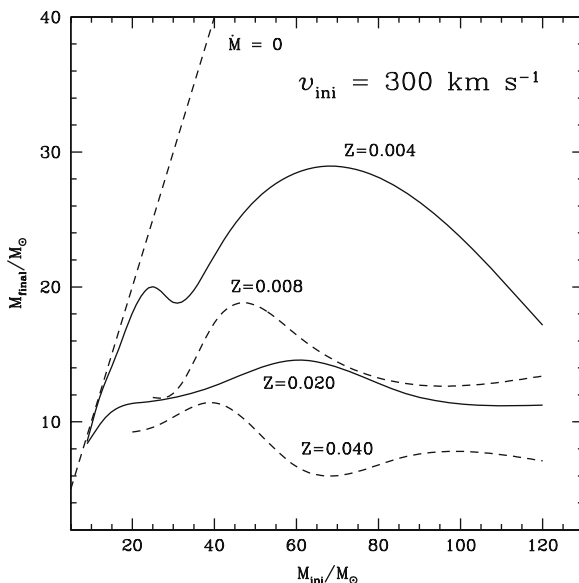
Fig. 28.12 Relation between the final and initial masses at different metallicities. From G. Meynet and the author [412]
