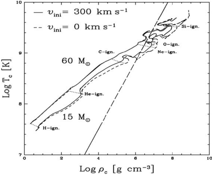
Fig. 28.4 Evolution of central conditions without and with rotation for Z = 0.02 models. The straight dashed line shows the electron degeneracy limit. From R. Hirschi et al. [251]
