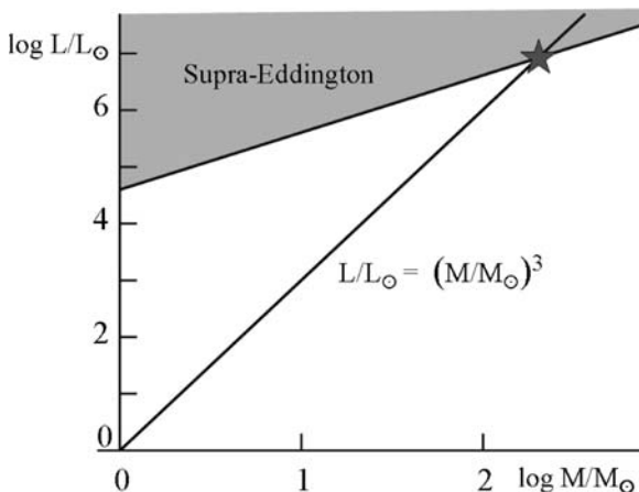
Fig. 3.6 The steeper line represents schematically the mass–luminosity relation, while the other line represents the Eddington luminosity as a function of mass for a value X = 0.70 , which gives \kappa_{\text{es}} = 0.34 \text{ cm}^2 \text{ g}^{-1} . The star at the intersection of the two lines provides a first rough approximation of the maximum stellar mass
