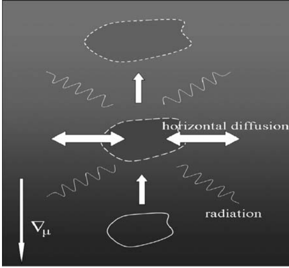
Fig. 12.6 Illustration of the role of the horizontal turbulence, which reduces the composition difference of the vertically moving eddies in a medium with a shear. Adapted from Talon & Zahn [562]
