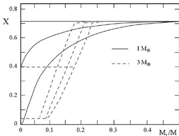
Fig. 25.14 Evolution of the distributions of hydrogen in stars of 1 and 3 M_{\odot} . Two stages of evolution are shown, at the middle and at the end of the H-burning phase. A convective core at 3 M_{\odot} creates a flat H profile near the center. Three cases are shown for 3 M_{\odot} : no overshooting, overshooting with d_{\text{over}}/H_P \approx 0.08 and twice larger (from left to right). Adapted from the author [336]
