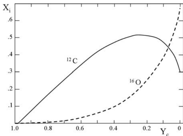
Fig. 26.5 Evolution of the carbon and oxygen abundances in the core of a 7 M_{\odot} during the He-burning phase. The mass fraction of ^{12}\text{C} and ^{16}\text{O} is given as a function of the central helium content Y_c
