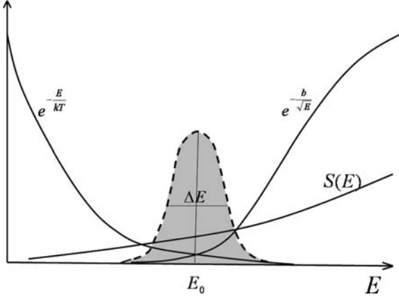
Fig. 9.5 Schematic representation of the various contributions to the reaction rate: on the left , the Maxwell distribution of the relative kinetic energies; on the right , the penetration factor of the potential barrier magnified by about 3 orders of magnitude. The Gamov peak is shown by the gray area, it is magnified by about 5 orders of magnitude. The astrophysical factor S(E) varies slowly
