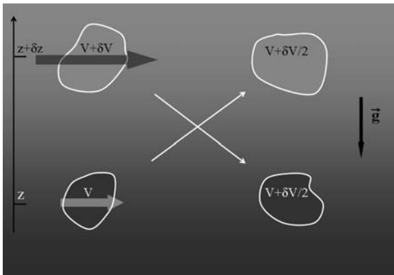
Fig. 12.4 Velocity exchanges during shear instability, as a result the velocities in the medium tend toward a local average. Adapted from Talon [556]
