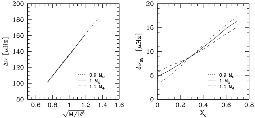
Fig. 16.15 Left : the mean large separation as a function of the square root of M/R^3 , with M and R expressed in solar units for star of different masses. Right : the small separation \delta\nu_{0,2} defined in Sect. 16.5.3 as a function of the central H content in mass fraction. Solar model with an initial X = 0.718 , Y = .268 , Z = 0.014 and \ell/H_p = 1.6 . From numerical models by P. Eggenberger [169]
