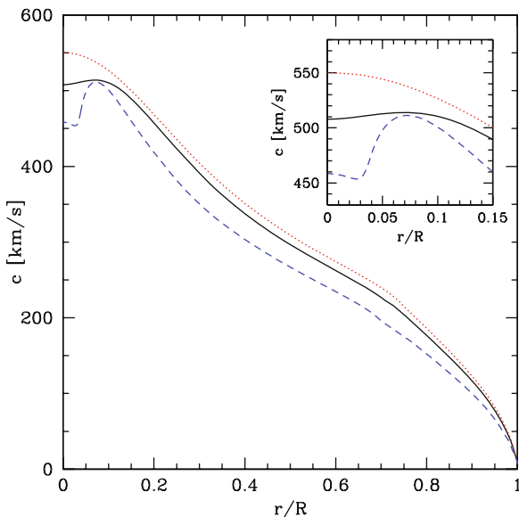
Fig. 16.11 The variations of the sound speed as a function of radius in models of a 1 M_{\odot} star at an age of 0.4, 4.57 and 9.8 Gyr indicated by the dotted, continuous and dashed lines, respectively. The initial composition is X = 0.718 , Y = 0.268 , Z = 0.014 . From P. Eggenberger [169]
