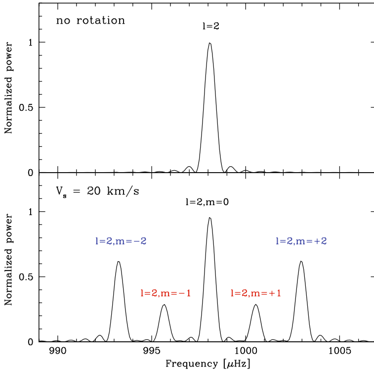
Fig. 16.19 Illustration of the rotational splitting: the power spectrum of an \ell = 2 mode for a 1.5 M_{\odot} star without rotation and with a solid body rotation of 20 \text{ km s}^{-1} . From P. Eggenberger [169]
