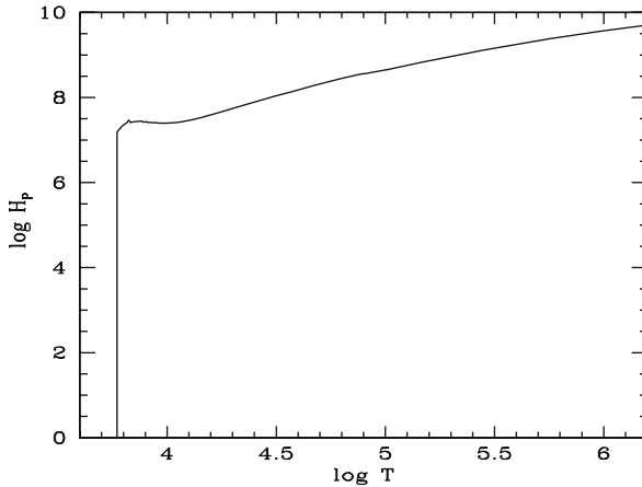
Fig. 5.1 The pressure scale height H_p in the outer solar layers. The value of \log(H_p) is shown as a function of \log T , where H_p is expressed in cm. T = 10^6 K at M_r/M_\odot = 0.995 , R/R_\odot = 0.846 , see also Fig. 7.2
