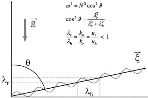
Fig. 17.1 Schematic illustration of the propagation of a gravity wave
