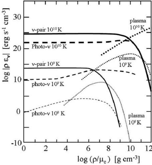
Fig. 9.8 Neutrino emission rates from pair annihilation, photo-neutrinos and plasma oscillations as functions of density for different temperatures. Each process is represented by lines of different types, thicker for higher T . For T = 10^8 K there is no pair annihilation process. Adapted from N. Itoh et al. [269]
