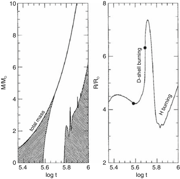
Fig. 20.4 Left: evolution of the convective zones (in gray) in a star with a growing mass. Initially the star is fully convective and then convection recedes from the center to finally disappear in the whole star. The star is then fully radiative and at higher masses a convective core appears. Right: corresponding evolution of the radius. From P. Bernasconi and the author [44]
