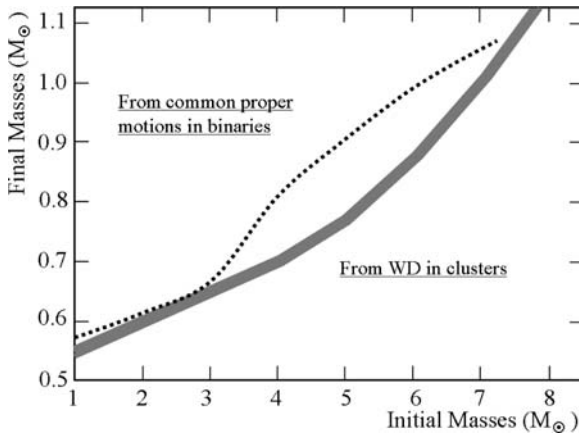
Fig. 26.21 Observational relation between initial and final masses based on white dwarfs in open clusters from V. Weidemann [607] and on WD with proper motions in binaries from S. Catalan [98]
