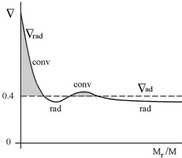
Fig. 5.4 Schematic representation of the course of \nabla_{\text{rad}} and \nabla_{\text{ad}} as a function of the mass coordinate in a massive star. Convection occurs in gray areas
