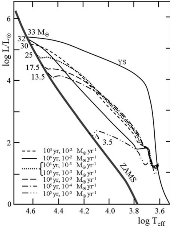
Fig. 22.8 Birthlines of massive stars for various accretion rates parametrized by (19.26) \dot{M}(t) = \dot{M}_0 \frac{e}{\tau_0} t e^{-\frac{t}{\tau_0}} of S. Schmeja and S.R. Klessen [518]. The values of \tau_0 and \dot{M}_0 in M_\odot \text{ yr}^{-1} are indicated, as well as the final masses on the ZAMS. These tracks do not account for the optically thick infalling matter. The track YS is from H.W. Yorke and C. Sonnhalter [630]; it accounts for the radiative transfer in the accretion flow and for the accretion luminosity. L = 10^4 L_\odot is reached in 10^4 yr. From C. Peter [464]
