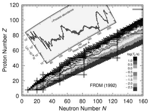
Fig. 28.17 Z vs. N plane of protons vs. neutron numbers. The valley of stability is formed by the black squares denoting \beta -stable nuclei. The gray region in the main graph shows calculated half-life with respect to \beta^- decay. The jagged black line gives the right-hand boundary of the region of known nuclei. The thick gray line shows the r-process path for typical stellar conditions. The solar r-process abundances shown in the insert are plotted vs. the mass number A , whose axis is curved slightly to follow the line of \beta -stability. A line perpendicular to the valley of \beta -stability and originating at a particular mass value crosses the A axis of the insert plot at right angles at this value and also passes through the point giving the abundance for this A value. The double lines show the magic numbers N and Z . Courtesy from P. Möller
