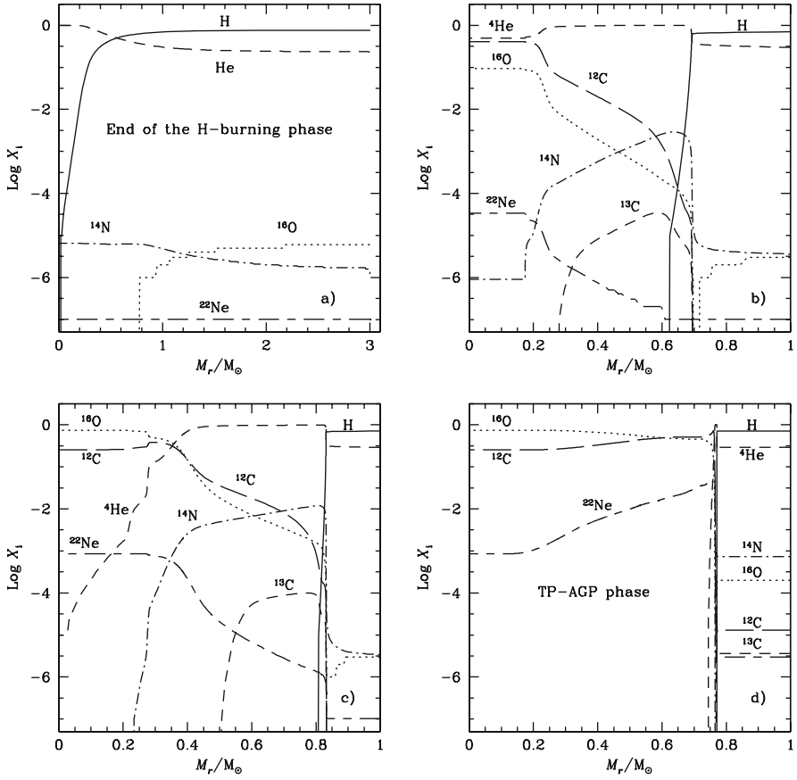
Fig. 26.22 Element abundances in a rotating 3 M_{\odot} model at Z = 10^{-5} . The initial velocity on the ZAMS is 300 \text{ km s}^{-1} , which corresponds to an average velocity during the MS of \sim 230 \text{ km s}^{-1} . Panel (a) shows the chemical structure at the end of the MS phase. Panels (b) and (c) at the middle and at the end of the core He-burning phase. The structure after the first five pulses along the TP-AGB branch is shown in panel (d). From G. Meynet and the author [410]
