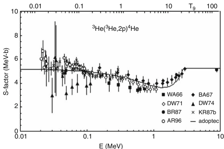
Fig. 9.4 Various empirical determinations of the factor S(E) as a function of energy for the reaction {}^3\text{He}({}^3\text{He}, 2p){}^4\text{He} . The raise at low energies is due to the screening factor. From the Nacre Library, European Compilation of Reaction Rates for Astrophysics, with permission
