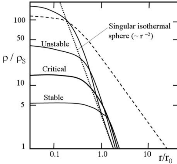
Fig. 18.3 Examples of density profiles as a function of the radius in Bonnor–Ebert spheres, i.e., truncated isothermal polytrope in a medium with an ambient pressure P_{\text{ext}} . The quantity \varrho_s is the surface density. The surface is at about 2r_0 , defined as r_0 = c_s^2(2\pi G P_{\text{ext}})^{-1/2} . Distributions more concentrated than the critical one are unstable and collapse, those less concentrated are stable. The singular solution ( dotted line ) is the limiting curve with \varrho \sim r^{-2} and an infinite central density [528]. The broken line illustrates the distribution in infalling regions above the shock, with \varrho \sim r^{-3/2} (18.44). Adapted from McLaughlin & Pudritz [395]
