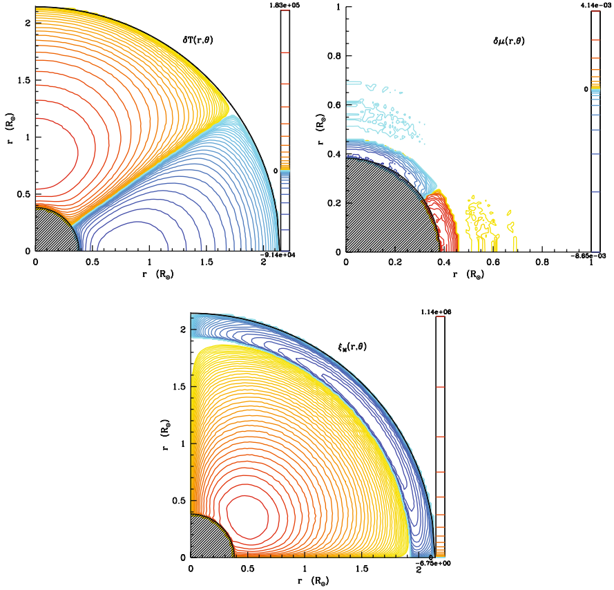
Fig. 11.5 The T excesses \tilde{T} P_2(\cos \vartheta) , \mu excesses \tilde{\mu} P_2(\cos \vartheta) and circulation currents in a 5 M_\odot star with Z = 0.0005 , v_{\text{ini}} = 300 \text{ km s}^{-1} , an age of 3.45 \times 10^7 \text{ yr} and X_c = 0.53 . The inner cell turns counterclockwise and the external clockwise. The T excesses are +1.8 \times 10^5 \text{ K} in the interior close to the polar axis and -9.1 \times 10^4 \text{ K} in the inner equatorial region, they are smaller near the surface. \mu excesses only occur close to the core, they are positive near the equator, consistently with the rotation of the inner cell. Courtesy T. Decressing [153]
