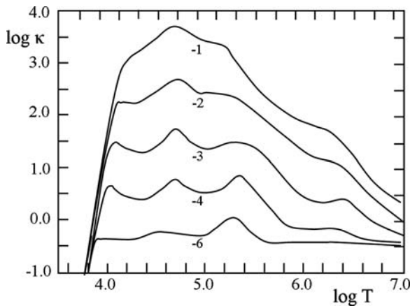
Fig. 8.5 Representation of the opacity as a function of \log T for different values of \log R , where R = \rho/T_6^3 . From Rogers & Iglesias [493]
